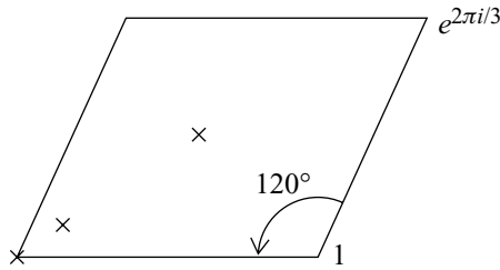
Fig. 25.1. Torus that admits a Z_3 symmetry, allowing an orbifold construction.
