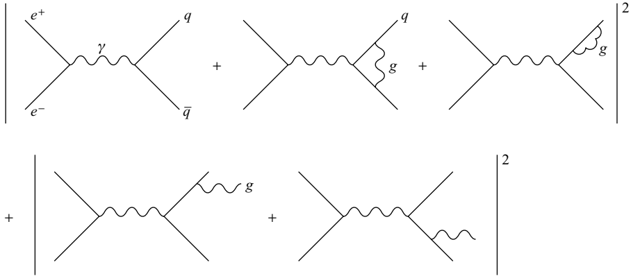
Fig. 3.6. Low-order contributions to e^+e^- annihilation.
