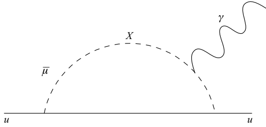
Fig. 11.6. Contribution to d_n in supersymmetric theories.
