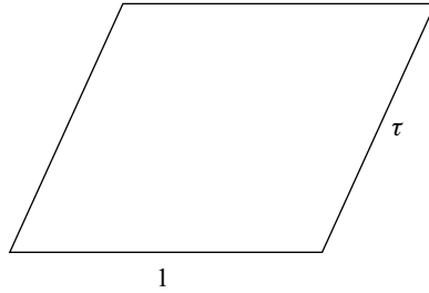
Fig. 21.2. A simple representation of a torus.
