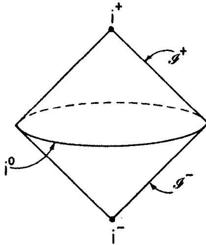
Fig. 11.2. The region \bar{O} of the Einstein static universe represented as two null cones joined at their base. This representation of \bar{O} is misleading since it shows i^0 as a 2-sphere rather than a point, but it often is much more convenient to use this representation for drawing spacetime diagrams than that of Figure 11.1.
