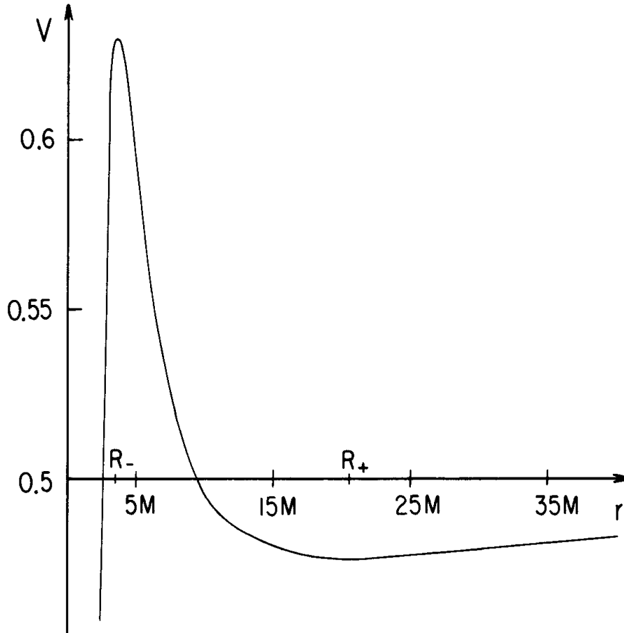
Fig. 6.4. The effective potential, V , for timelike geodesics in the case L^2 = 24M^2 . (Note that the scale of V is greatly expanded as compared with Fig. 6.3.)
