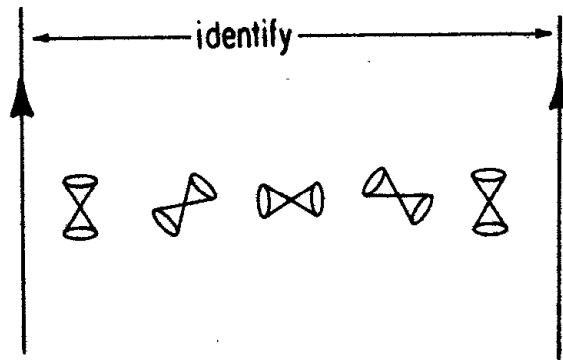
Fig. 8.1. A non-time-orientable spacetime.
