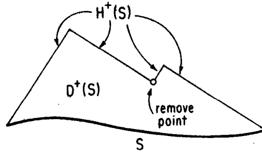
Fig. 8.11. A spacetime diagram showing the future domain of dependence, D^+(S) , and Cauchy horizon H^+(S) of a particular closed achronal set S in Minkowski spacetime with a point removed.
