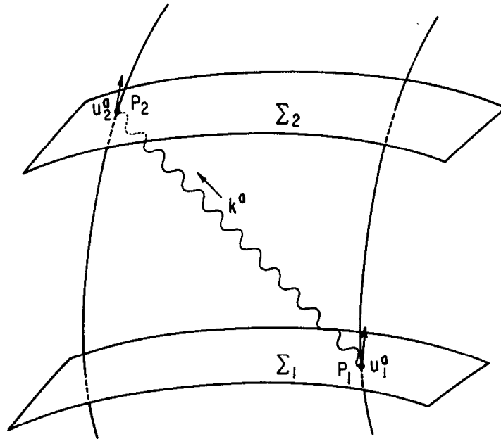
Fig. 5.5. A spacetime diagram showing the emission of a light signal at event P_1 and its reception at event P_2 .
