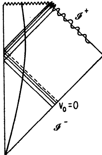
Fig. 14.3. A conformal diagram of a spherically symmetric spacetime in which gravitational collapse to a Schwarzschild black hole occurs, showing the oscillations of a wave which behaves as e^{-i\omega u} on \mathcal{I}^+ . If one propagates this wave backward into the past starting from \mathcal{I}^+ , the part of the wave which propagates through the collapsing matter will produce an “infinite blueshift” singularity—of the same nature as shown on the white hole horizon in Figure 14.2—at advanced time v_0 on \mathcal{I}^- .
