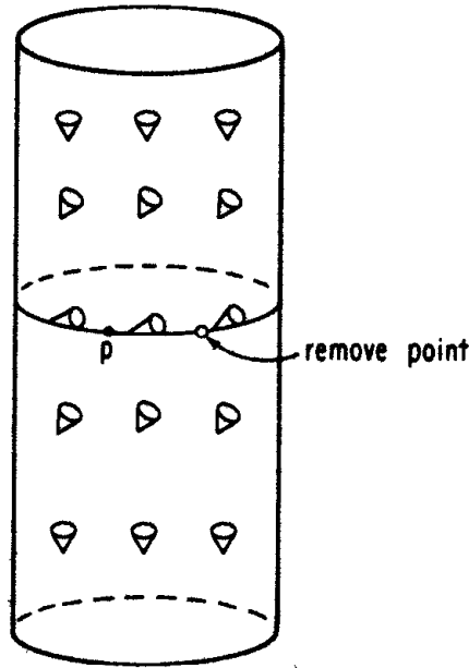
Fig. 8.8. A spacetime which violates strong causality. The light cones “tip over” sufficiently that the curve drawn through p is a null geodesic (which, however, is not a closed curve because of the point removed from the manifold). There exist no closed causal curves in this spacetime, but there are causal curves through p which come “arbitrarily close” to intersecting themselves.
