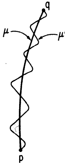
Fig. 9.5. A smooth timelike curve \mu from p to q . Arbitrarily close to \mu in the topology of C(p, q) is a smooth timelike curve \mu' with total elapsed proper time arbitrarily close to zero.
