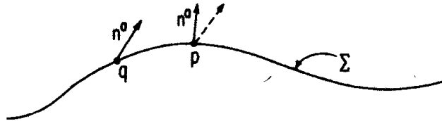
Fig. 10.3. A spacetime diagram illustrating the notion of the extrinsic curvature of a hypersurface \Sigma . The dashed arrow at p represents the parallel transport of the normal vector, n^a , at q along a geodesic connecting q to p . The failure of this vector to coincide with n^a at p corresponds intuitively to the bending of \Sigma in the spacetime in which it is embedded. The formula K_{ab} = h_a{}^c \nabla_c n_b shows that K_{ab} directly measures this failure of the two vectors at p to coincide for q near p .
