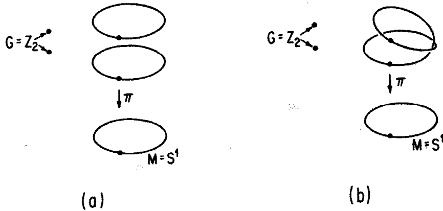
Fig. 13.3. (a) The trivial principal fiber bundle Z_2 \times S^1 . (b) The principal bundle (S^1, Z_2, S^1, \phi) constructed in the text.
