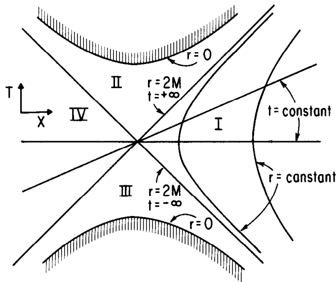
Fig. 6.9. The Kruskal extension of Schwarzschild spacetime.
