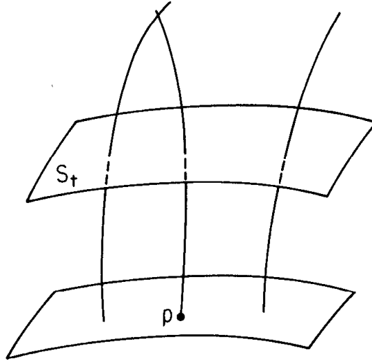
Fig. 3.4. The construction of Gaussian normal coordinates starting from the hypersurface S . The geodesics orthogonal to S eventually may cross, but until they do, Gaussian normal coordinates are well defined and the surfaces, S_t , of constant t remain orthogonal to the geodesics.
