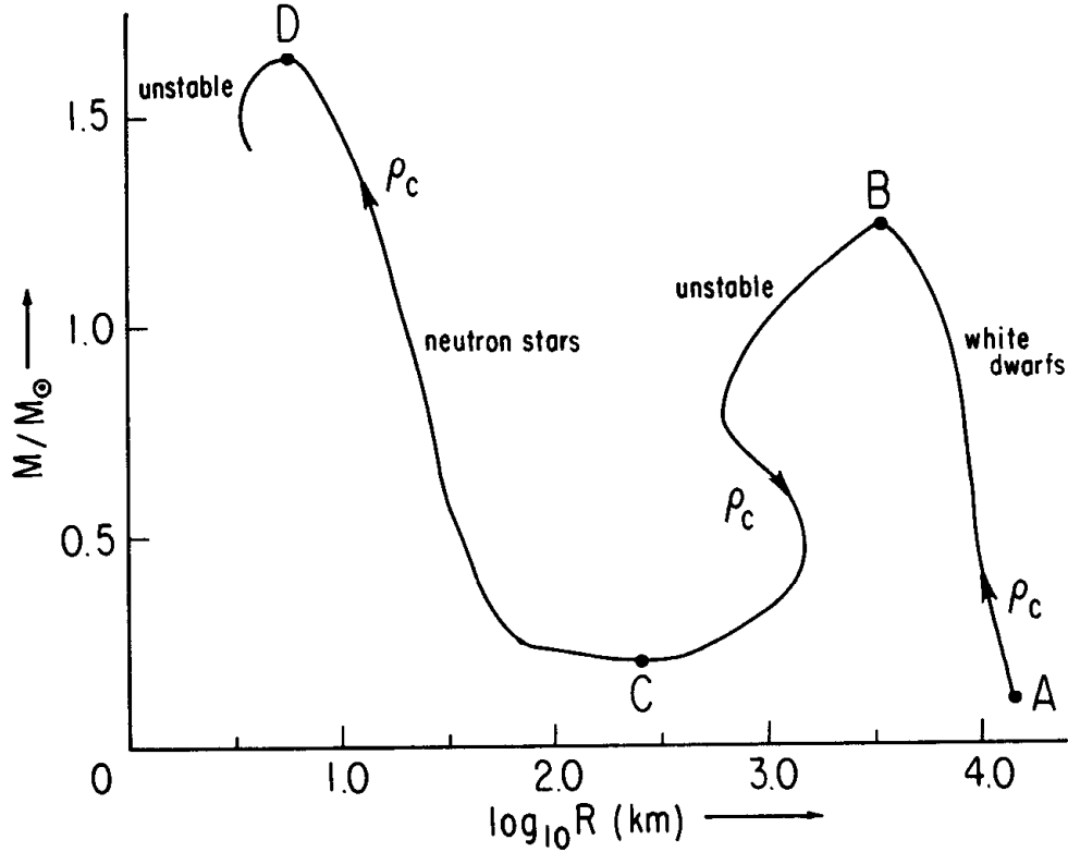
Fig. 6.1. The equilibrium configurations of cold matter. Given an equation of state, P = P(\rho) , an equilibrium configuration is uniquely determined by the value of the central density \rho_c . The masses and radii of these configurations are shown here for values of \rho_c ranging from \sim 10^5 \text{ g cm}^{-3} at point A to \sim 10^{17} \text{ g cm}^{-3} beyond point D. In the white dwarf regime, the values of M and R depend somewhat upon the assumed composition of the star. In the neutron star regime, the values of M and R depend greatly upon assumptions about the state of matter as well as assumptions about the interactions between the fundamental constituents of matter. In this latter regime, the figure is only a rough sketch of the qualitative features found for most equations of state.
