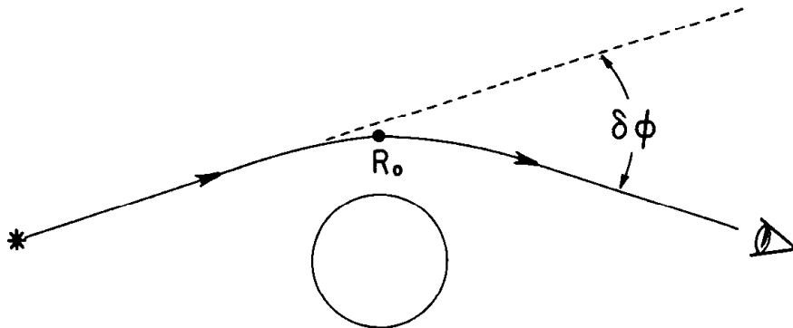
Fig. 6.6. Diagram illustrating the “bending of light” effect.
