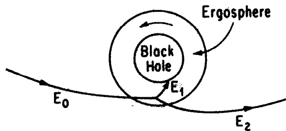
Fig. 12.7. A diagram illustrating the Penrose process for extracting energy from a Kerr black hole.
