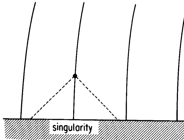
Fig. 5.6. The causal structure of the Robertson-Walker solutions near the big-bang singularity. Particle horizons exist since an observer cannot “see” all other isotropic observers in the universe.
