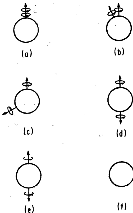
Fig. 13.1. A diagram illustrating how a rotation of a sphere by 4\pi about a given axis can be continuously deformed to no rotation. We break up the 4\pi -rotation into two 2\pi -rotations and continuously change the axis of the second 2\pi -rotation until it is opposite the axis of the first rotation, as shown in the sequence (a)–(d). Then we continuously decrease the angle of both rotations to zero, as shown in the sequence (d)–(f).
