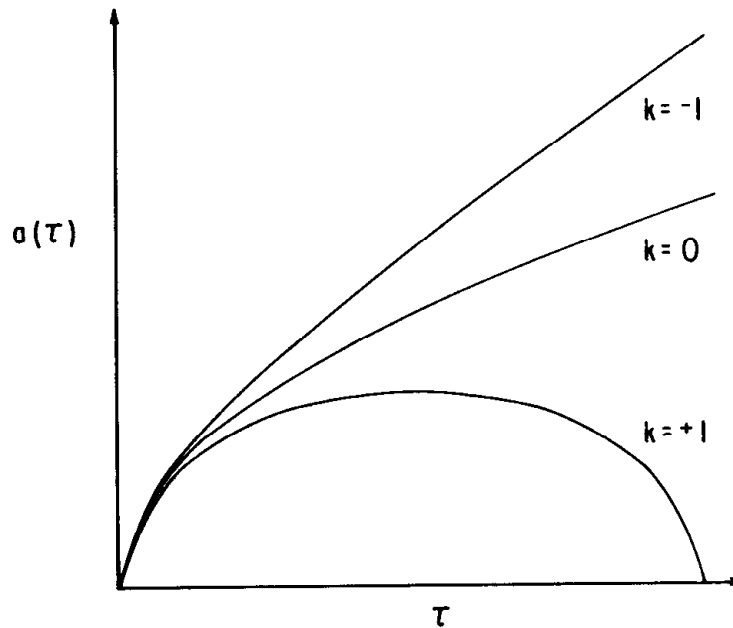
Fig. 5.3. The dynamics of dust-filled Robertson-Walker universes.
