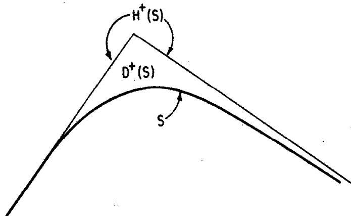
Fig. 8.12. A spacetime diagram showing D^+(S) and H^+(S) for a particular closed achronal set S in Minkowski spacetime. Here S is “asymptotically null” to the right and becomes “exactly null” to the left. This example shows that H^+(S) can intersect S even if \text{edge}(S) = \emptyset .
