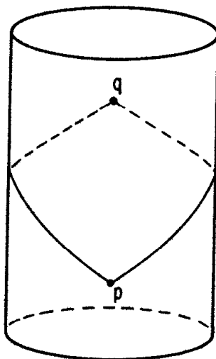
Fig. 8.5. A spacetime diagram of a two-dimensional flat spacetime with topology \mathbb{R} \times S^1 . The null geodesic generators of I^+(p) have q as a future endpoint.
