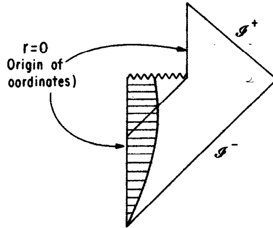
Fig. 14.4. A conformal diagram of a spacetime in which a black hole is produced by the collapse of matter and “evaporates” as a result of the particle creation process.
