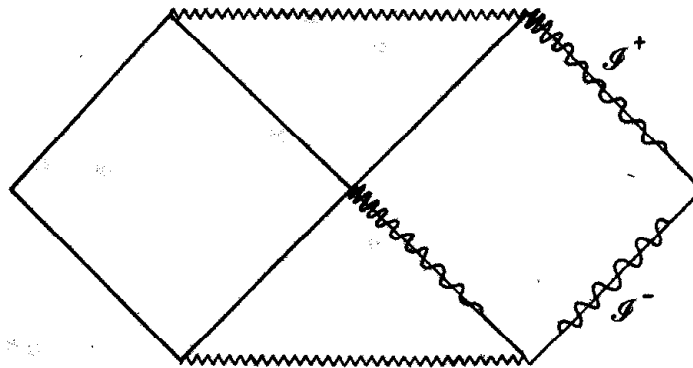
Fig. 14.2. A conformal diagram of the extended Schwarzschild spacetime (see Fig. 12.3) showing the oscillations of a wave of frequency \omega , i.e., \mathcal{L}_\xi \phi = -i\omega \phi . The apparent increase in oscillation frequency shown in the figure on \mathcal{I}^+ at late retarded time (which also occurs on \mathcal{I}^+ at early retarded time and on \mathcal{I}^- at late and early advanced times) is merely an artifact of the conformal diagram caused by the behavior of the conformal factor there. However, the increase in frequency shown on the white hole horizon near its crossing point with the black hole horizon represents a physical “infinite blueshift” singularity of the wave.
