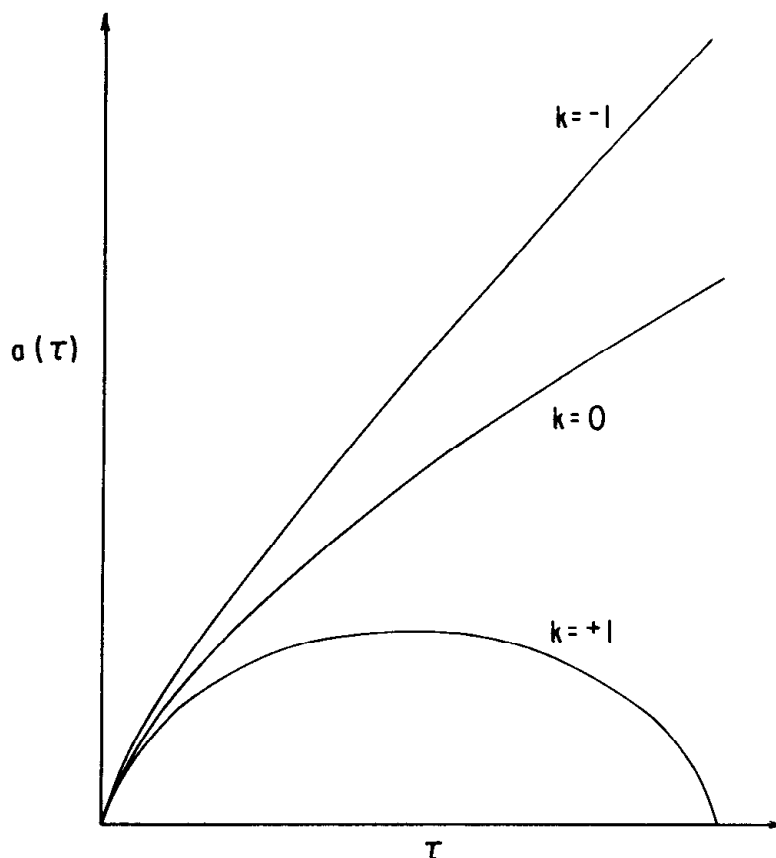
Fig. 5.4. The dynamics of radiation-filled Robertson-Walker universes.
