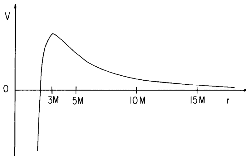
Fig. 6.5. The effective potential, V , for null geodesics.
