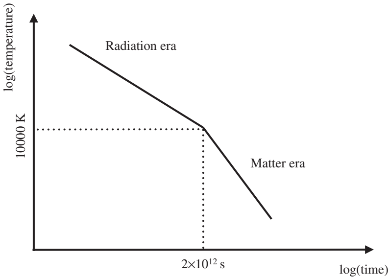
Figure 11.1 A schematic illustration of the temperature–time relation, assuming \Omega_0 = 0.3 and h = 0.7 . When the radiation era ends the expansion rate increases and the temperature cools more quickly.
