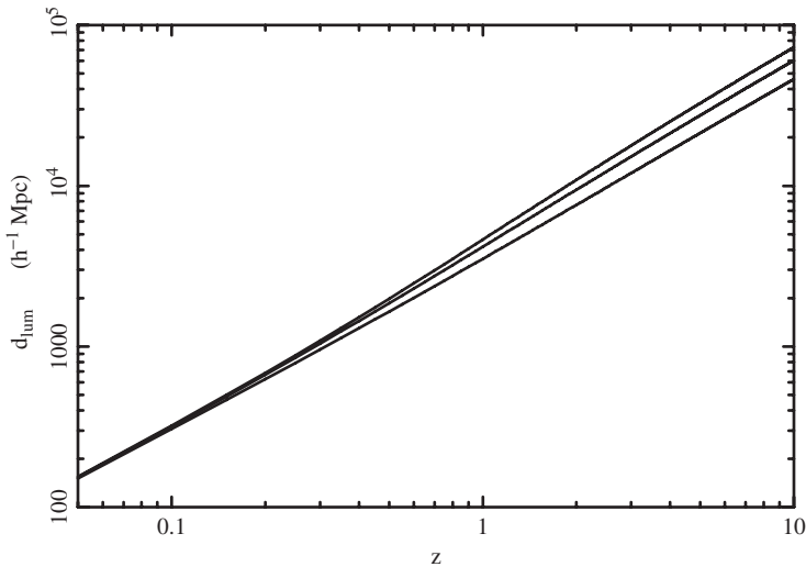
Figure A2.3 The luminosity distance as a function of redshift is plotted for three different spatially-flat cosmologies with a cosmological constant. From bottom to top, the lines are \Omega_0 = 1, 0.5 and 0.3 respectively. Notice how weak the dependence on cosmology is even to high redshift. It turns out that open universe models with no cosmological constant have an even weaker dependence.
