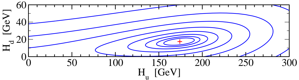
Figure 8.1: A contour map of the Higgs potential, for a typical case with \tan\beta \approx -\cot\alpha \approx 10 . The minimum of the potential is marked by +, and the contours are equally spaced equipotentials. Oscillations along the shallow direction, with H_u^0/H_d^0 \approx 10 , correspond to the mass eigenstate h^0 , while the orthogonal steeper direction corresponds to the mass eigenstate H^0 .
