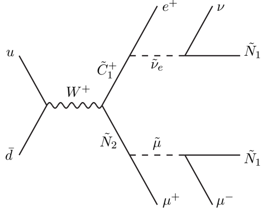
Figure 10.4: A complete Feynman diagram for a clean (no high- p_T hadronic jets) triplepton event at a hadron collider, from production of an on-shell neutralino and a chargino, with subsequent leptonic decays, leading in this case to \mu^+\mu^-e^+ + \cancel{E}_T .
