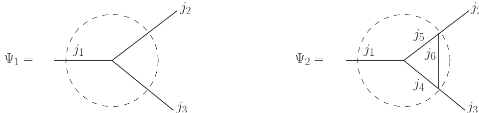
Figure 7. Two spin networks states \Psi_1 and \Psi_2 which differ only in a small neighborhood.
