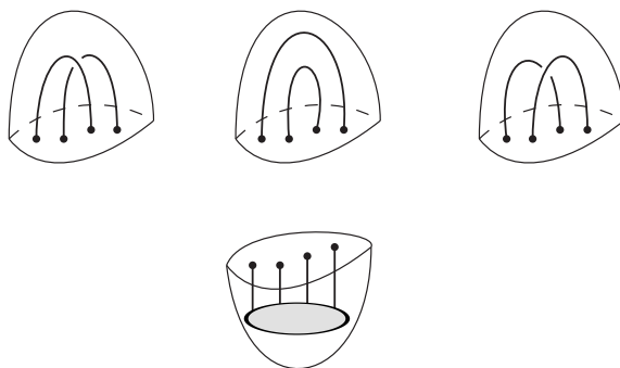
Figure 3. Examples of knots in S^3 . They coincide in the “southern hemisphere” of S^3 but differ in the “northern hemisphere”
