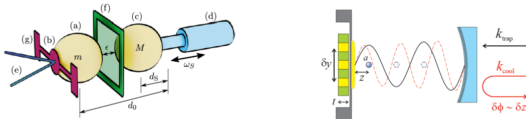
Figure 6. Optomechanical experiments to test gravity: Left Panel: A test-mass m (a) is loaded on a micromechanical device (b). A source mass M (c) is located at a COM distance d_0 from the test mass and is modulated through a drive motor (d) with maximum amplitude d_s . The displacement of the test mass cantilever is read out optically (e). Other, non-gravitational forces are further suppressed by a shielding membrane (f). (g) labels the mounting support structure. Picture and caption taken from [228]. Right Panel. Levitated optomechanics proposal and experiment to test gravity. Proposed experimental geometry. A sub-wavelength dielectric microsphere of radius a is trapped with light in an optical cavity. The sphere is positioned at an anti-node occurring at distance z from a gold-coated SiN membrane. Light of a second wavelength \lambda_{cool} = 2\lambda_{trap}/3 is used to simultaneously cool and measure the center-of-mass motion of the sphere. The sphere displacement \delta z results in a phase shift \delta\phi in the cooling light reflected from the cavity. For the short-range gravity measurement, a source mass of thickness t with varying density sections is positioned on a movable element behind the mirror surface that oscillates harmonically with an amplitude \delta y . The source mass is coated with a thin layer of gold to provide an equipotential. Reprinted figure and caption with permission from [240]. Copyright 2010 by the American Physical Society.
