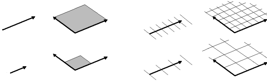
Figure 4: Two vectors (far left) with the same direction and different magnitude differ in their length, while two bivectors (left) differ in their area. The magnitude of k -forms is a density, and can be represented by interval lines. A 1-form (right) has a direction, just like a vector, but the spacing of interval lines represents its magnitude. A 2-form (far right) defines a plane, just like a bivector does, and once again the magnitude is represented by the spacing of interval lines. In all cases, the greater magnitude object is on the top row.
