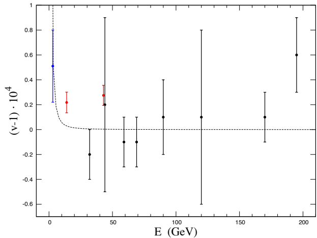
FIG. 3. fit with the special-relativistic-tachyon hypothesis
