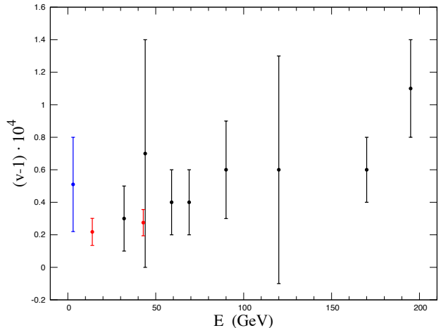
FIG. 1. The result for the speed of \mu neutrinos reported in OPERA (red), FERMILAB07(blue) and FERMILAB79 (black)
