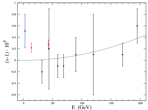
FIG. 6. fit with the DSR-quadratic case
