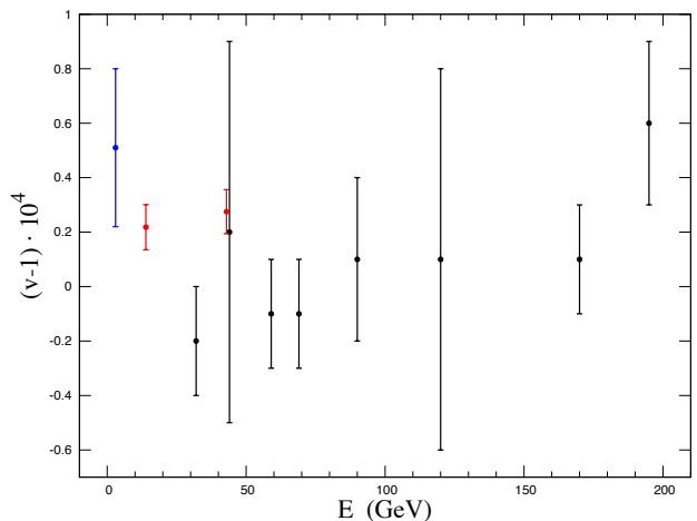
FIG. 2. As in fig.1 but taking into account the bias correction of Ref. [3]
