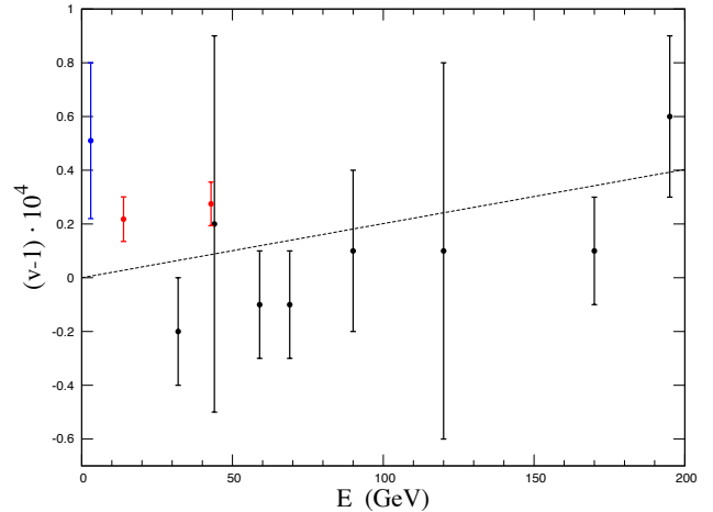
FIG. 5. fit with the DSR-linear case
