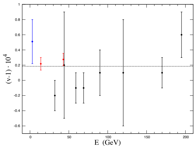
FIG. 4. fit with the Coleman-Glashow hypothesis
