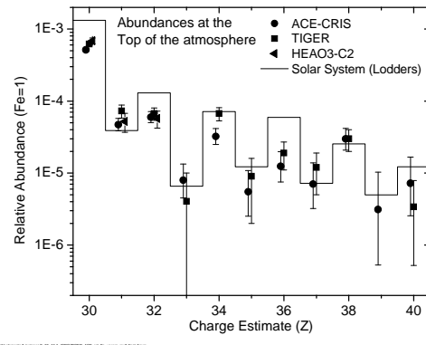
Figure 2. Element abundances relative to Fe. Data points show GCR abundances outside the atmosphere and histogram shows SS abundances.
