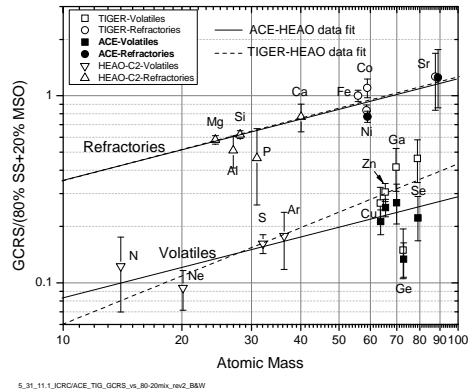
Figure 3. GCR Source abundances relative to the 80%-20% mix described in the text.
