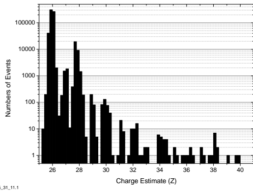
Figure 1. Observed number of events vs assigned charge.
