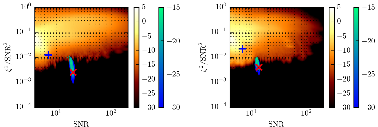
FIG. 6. Two projections of parameters in the multi-dimensional likelihood ratio ranking for GstLAL (left: H1, right: L1). The relative positions of GW150914 (red cross) and LVT151012 (blue plus) are indicated in the \xi^2/\rho^2 vs matched-filter SNR plane. A warm colormap is used for the log of the probability density function consisting of only background, non-coincident triggers. A cool colormap is used for the log of the probability density function consisting of both non-coincident and coincident triggers, including candidate events. The distribution of both background and coincident triggers (represented by the cool colormap) has been masked to only show regions which are not consistent with the background. The parameters of GW150914 reside in the only region where the probability density function differs, indicating that it is a special population of triggers not consistent with the noise. Rather than showing the \theta_i bins in which GW150914 and LVT151012 were found, \theta_i has been marginalized over to demonstrate that no background triggers from any bin had the parameters of GW150914.
