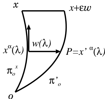
FIG. 8: The path defining the connection derivative.
