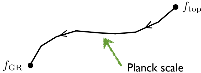
Figure 1: The conjectural RG flow
