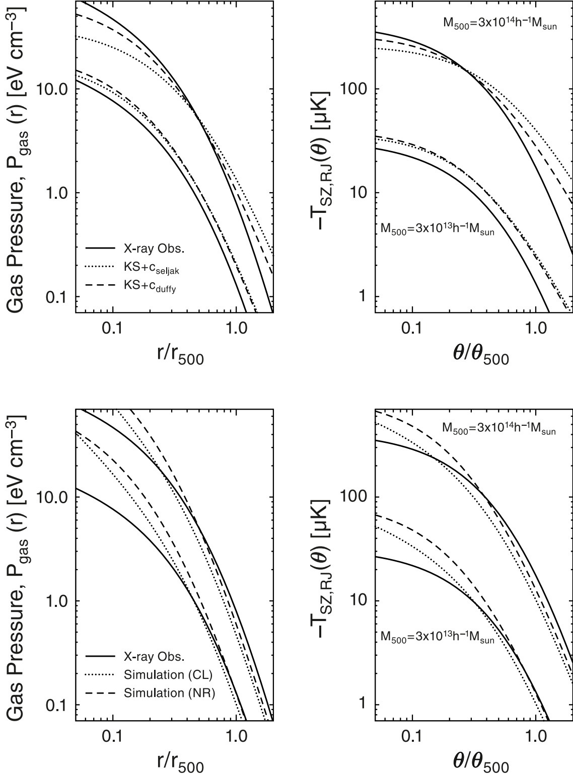
FIG. 16.— Gas pressure profiles of clusters of galaxies, P_{\text{gas}}(r) , at z = 0.1 , and the projected profiles of the SZ effect, \Delta T_{\text{SZ}}(\theta) (Rayleigh-Jeans temperature in \mu\text{K} ). (Top Left) The gas pressure profiles. The upper and bottom set of curves show M_{500} = 3 \times 10^{14} and 3 \times 10^{13} h^{-1} M_{\odot} , respectively. The horizontal axis shows radii scaled by the corresponding r_{500} = 0.78 and 0.36 h^{-1} \text{Mpc} , respectively. The solid lines show P_{\text{gas}}(r) = P_e(r)/0.518 derived from X-ray observations (Arnaud et al. 2009), while the dotted and dashed lines show P_{\text{gas}}(r) predicted from hydrostatic equilibrium (Komatsu & Seljak 2001) with NFW concentration parameters of Seljak (2000) and Duffy et al. (2008), respectively. (Top Right) The projected SZ profiles computed from the corresponding curves in the top left panel and equation (87). The horizontal axis shows angular radii scaled by \theta_{500} = r_{500}/D_A , which is 10 and 4.7 arcmin for M_{500} = 3 \times 10^{14} and 3 \times 10^{13} h^{-1} M_{\odot} , respectively. (Bottom Left) Same as the top left panel, but the dotted and dashed lines show P_{\text{gas}}(r) predicted from “Cooling+Star Formation” and “Non-radiative” simulation runs by Nagai et al. (2007). (Bottom Right) Same as the top right panel, but the dotted and dashed lines are computed from the corresponding curves in the bottom left panel and equation (87).
