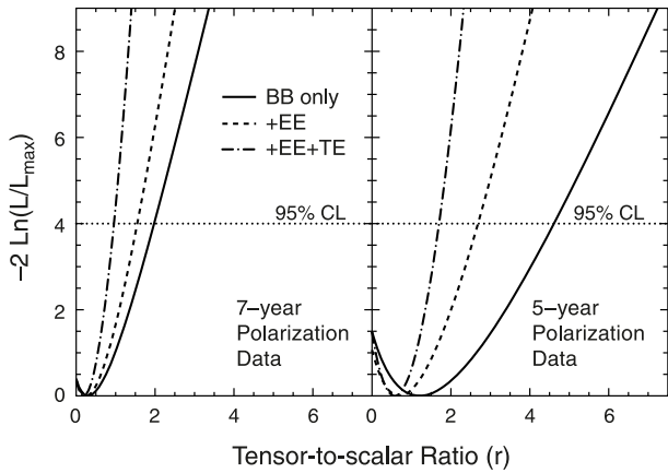
FIG. 8.— Limits on the tensor-to-scalar ratio, r , from the polarization data (BB, EE and TE) alone. All the other cosmological parameters, including the optical depth, are fixed at the 5-year best-fit \Lambda CDM model (Dunkley et al. 2009). The vertical axis shows -2\ln(L/L_{\max}) , where L is the likelihood and L_{\max} is the maximum value. This quantity may be interpreted as the standard \chi^2 , as the likelihood is approximately a Gaussian near the maximum; thus, -2\ln(L/L_{\max}) = 4 corresponds to the 95.4% CL limit. The solid, dashed and dot-dashed lines show the likelihood as a function of r from the BB-only, BB+EE, and BB+EE+TE data. (Left) The 7-year polarization data. We find r < 2.1 , 1.6, and 0.93 (95.4% CL) from the BB-only, BB+EE, and BB+EE+TE data, respectively. (Right) The 5-year polarization data. We find r < 4.7 , 2.7, and 1.6 (95.4% CL) from the BB-only, BB+EE, and BB+EE+TE data, respectively.
