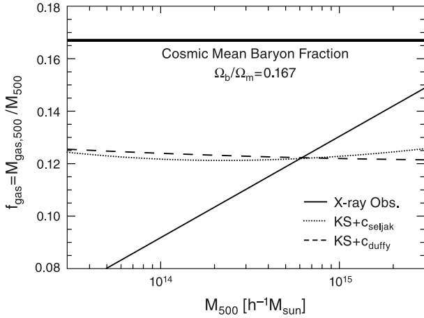
FIG. 17.— Gas mass fraction as a function of M_{500} . The thick horizontal line shows the cosmic mean baryon fraction, \Omega_b/\Omega_m = 0.167 . The solid line shows the gas mass fraction, f_{\text{gas}} = M_{\text{gas},500}/M_{500} , derived from X-ray observations (Vikhlinin et al. 2009a), while the dotted and dashed lines show f_{\text{gas}} predicted from hydrostatic equilibrium (Komatsu & Seljak 2001) with NFW concentration parameters of Seljak (2000) and Duffy et al. (2008), respectively.
