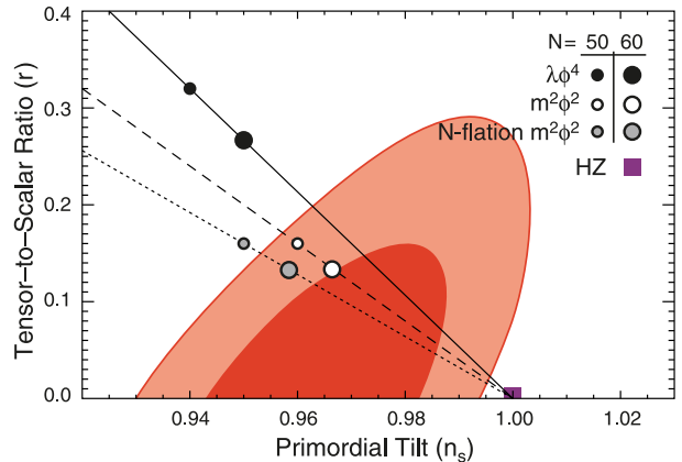
FIG. 19.— Two-dimensional joint marginalized constraint (68% and 95% CL) on the primordial tilt, n_s , and the tensor-to-scalar ratio, r , derived from the data combination of WMAP +BAO+ H_0 . The symbols show the predictions from “chaotic” inflation models whose potential is given by V(\phi) \propto \phi^\alpha (Linde 1983), with \alpha = 4 (solid) and \alpha = 2 (dashed) for single-field models, and \alpha = 2 for multi-axion field models with \beta = 1/2 (dotted; Easter & McAllister 2006).
