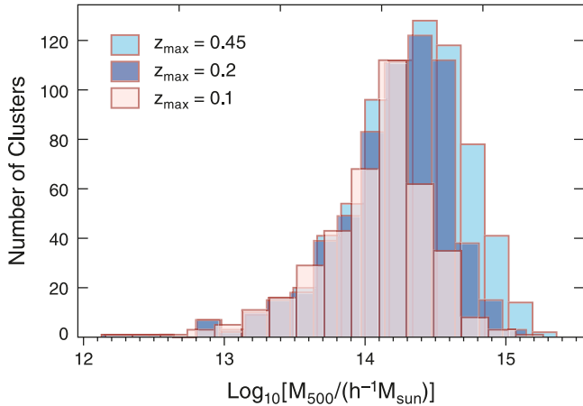
FIG. 18.— Distribution of M_{500} estimated from clusters in the catalog using the measured X-ray luminosities in 0.1–2.4 keV band, L_X , and equations (89) and (C2). The light blue, dark blue, and pink histograms show z_{\max} = 0.45 , 0.2, and 0.1, respectively.
