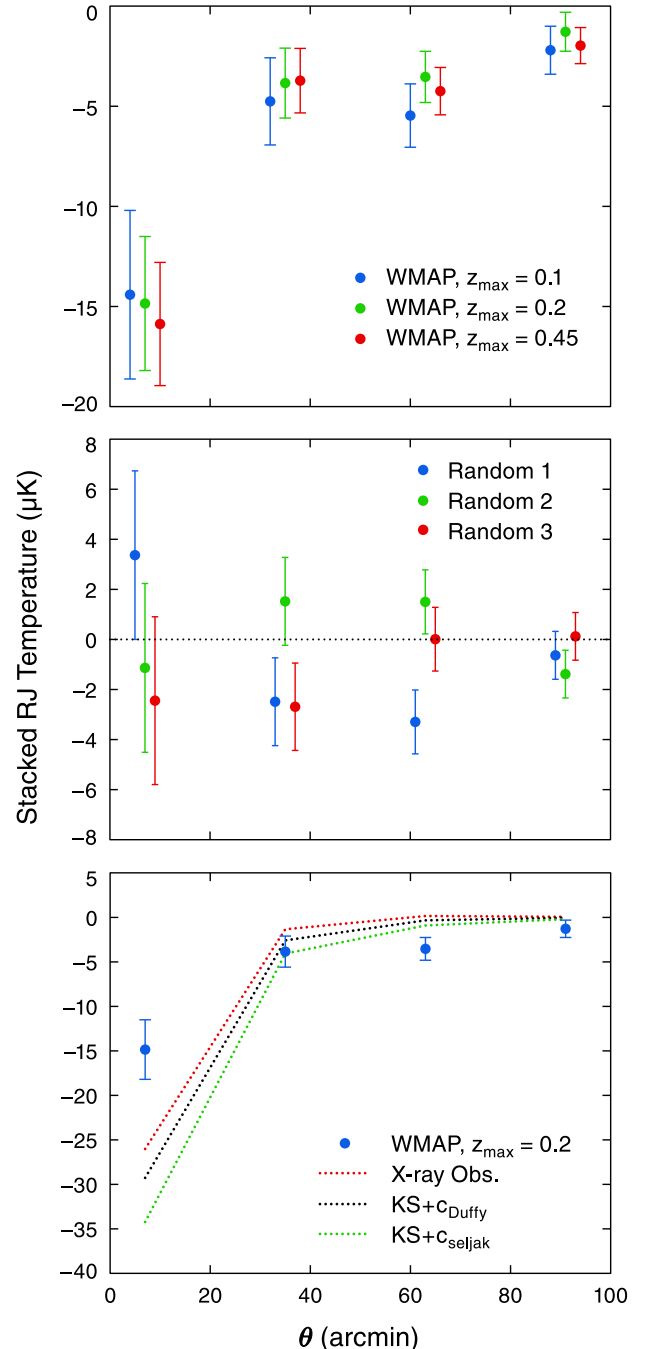
FIG. 15.— Average temperature profile of the SZ effect from the stacking analysis, in units of the Rayleigh-Jeans (RJ) temperature ( \mu\text{K} ), at \theta = 7, 35, 63 , and 91 arcmin. The V- and W-band data are combined using the optimal estimator. (Top) The SZ effect measured from the locations of clusters of galaxies. The results with three different maximum redshifts, z_{\text{max}} = 0.1 (blue; left), 0.2 (green; middle), and 0.45 (red; right), are shown. The error bars include noise due to the CMB fluctuation, and thus are correlated (see equation (82) for the correlation matrix). (Middle) A null test showing profiles measured from random locations on the sky (for z_{\text{max}} = 0.2 ; the number of random locations is the same as the number of clusters used in the top panel). Three random realizations are shown. Our method does not produce biased results. (Bottom) The measured profile ( z_{\text{max}} = 0.2 ) is compared with the model profiles derived from X-ray observations (Arnaud et al. 2009) and theoretically calculated from hydrostatic equilibrium (Komatsu & Seljak 2001) with two different concentration parameters. Note that the model profiles are calculated also for z_{\text{max}} = 0.2 but have not been multiplied by the best-fitting normalization factors given in Table 12.
