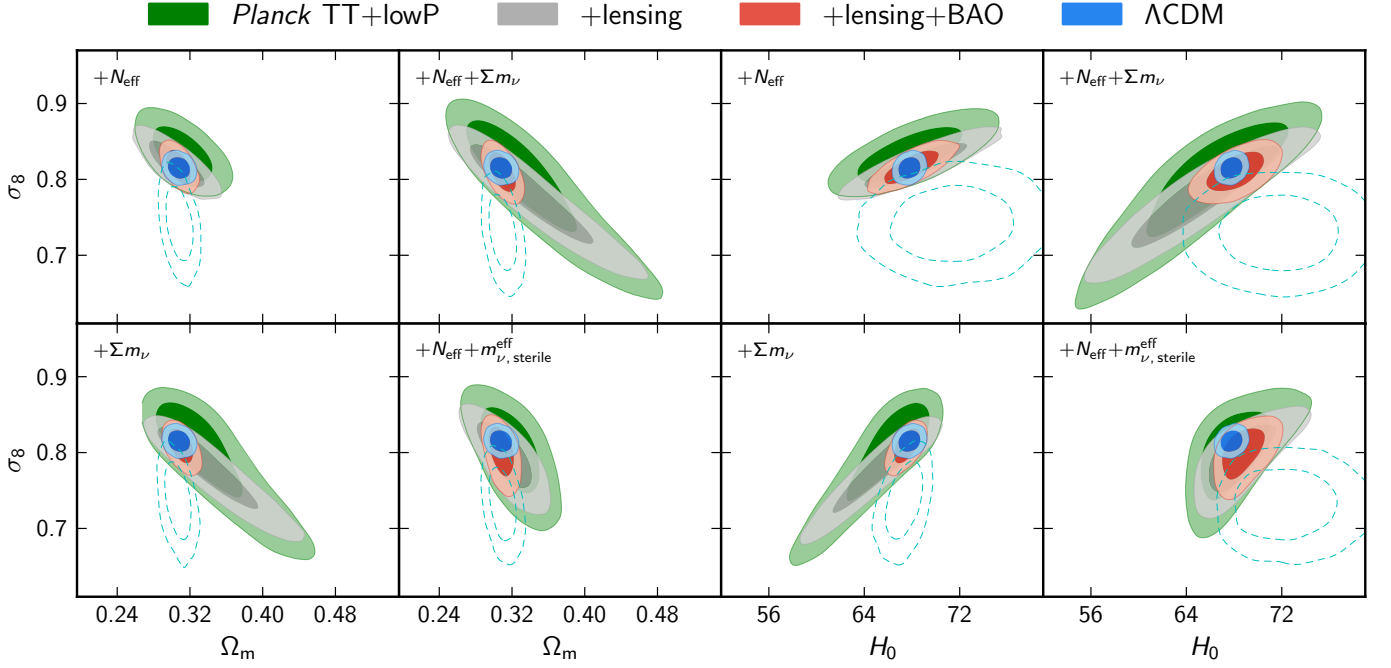
Fig. 33. 68% and 95% constraints from Planck TT+lowP (green), Planck TT+lowP+lensing (grey), and Planck TT+lowP+lensing+BAO (red) on the late-Universe parameters H_0 , \sigma_8 , and \Omega_m in various neutrino extensions of the base \Lambda CDM model. The blue contours show the base \Lambda CDM constraints from Planck TT+lowP+lensing+BAO. The dashed cyan contours show joint constraints from the H13 CFHTLenS galaxy weak lensing likelihood (with angular cuts as in Fig. 18) at fixed CMB acoustic scale \theta_{MC} (fixed to the Planck TT+lowP \Lambda CDM best fit) combined with BAO and the Hubble constant measurement of Eq. 30. These additional constraints break large parameter degeneracies in the weak lensing likelihood that would otherwise obscure the comparison with the Planck contours. (Priors on other parameters applied to the CFHTLenS analysis are as described in Sect. 5.5.2.)
