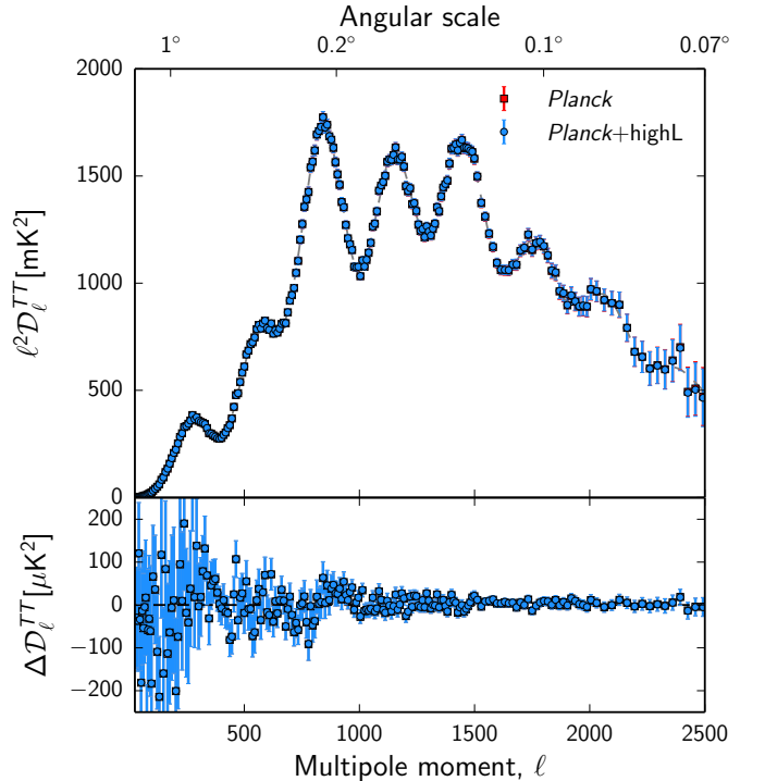
Fig. 10. Planck CMB power spectrum marginalized over foregrounds (red), including a prior on the thermal and kinetic SZ power. The inclusion of the full higher resolution ACT and SPT data (shown in blue) does not significantly decrease the errors.
