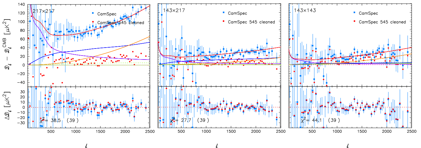
Fig. 2. Residual plots illustrating the accuracy of the foreground modelling. The blue points in the upper panels show the CamSpec 2015(CHM) spectra from after subtraction of the best-fit \Lambda CDM spectrum. The residuals in the upper panel should be accurately described by the foreground model. Major foreground components are shown by the solid lines, colour coded as follows: total foreground spectrum (red); Poisson point sources (orange); clustered CIB (blue); thermal SZ (green); and Galactic dust (purple). Minor foreground components are shown by the dotted lines, colour-coded as follows: kinetic SZ (green); and tSZ \times CIB cross-correlation (purple). The red points in the upper panels show the 545 GHz-cleaned spectra (minus best-fit CMB as subtracted from the uncleaned spectra) that are fitted to a power-law residual foreground model, as discussed in the text. The lower panels show the spectra after subtraction of the best-fit foreground models. These agree to within a few (\mu\text{K})^2 . The \chi^2 values of the residuals of the blue points, and the number of bandpowers, are listed in the lower panels.
