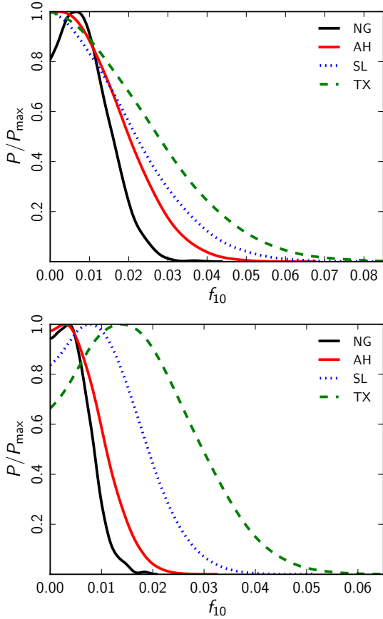
Fig. 46. Marginalized posterior distributions for the fractional contribution, f_{10} , of the defect contribution to the temperature power spectrum at \ell = 10 (see the text for the precise definition). Here we show the constraints for the Nambu-Goto cosmic strings (NG, solid black), field-theory simulations of Abelian-Higgs cosmic strings (AH, solid red), semi-local strings (SL, dotted blue), and global textures (TX, dashed green). The upper panel shows the 1D posterior for the Planck +lowP data, while constraints shown in the lower panel additionally use the TE and EE data.
