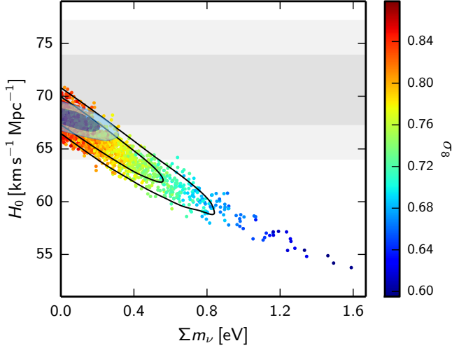
Fig. 29. Samples from the Planck TT+lowP posterior in the \Sigma m_\nu - H_0 plane, colour-coded by \sigma_8 . Higher \Sigma m_\nu damps the matter fluctuation amplitude \sigma_8 , but also decreases H_0 (grey bands show the direct measurement H_0 = (70.6 \pm 3.3) \text{ km s}^{-1} \text{ Mpc}^{-1} , Eq. 30). Solid black contours show the constraint from Planck TT+lowP+lensing (which mildly prefers larger masses), and filled contours show the constraints from Planck TT+lowP+lensing+BAO.
