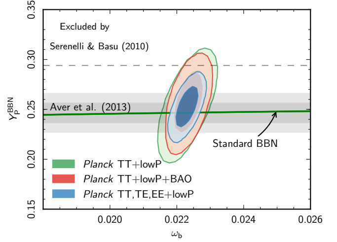
Fig. 38. Constraints in the \omega_b - Y_p^{\text{BBN}} plane from Planck and Planck+BAO, compared to helium abundance measurements. 68% and 95% contours are plotted for the CMB(+BAO) data combinations when Y_p^{\text{BBN}} is allowed to vary as an additional parameter to base \Lambda\text{CDM} . The horizontal band shows observational bounds on ^4\text{He} compiled by Aver et al. (2013) with 68% and 95% errors, while the dashed line at the top of the figure delineates the conservative 95% upper bound inferred from Solar helium abundance by Serenelli & Basu (2010). The green stripe shows the predictions of standard BBN for the primordial abundance of ^4\text{He} as a function of the baryon density. Both BBN predictions and CMB results assume N_{\text{eff}} = 3.046 and no significant lepton asymmetry.
