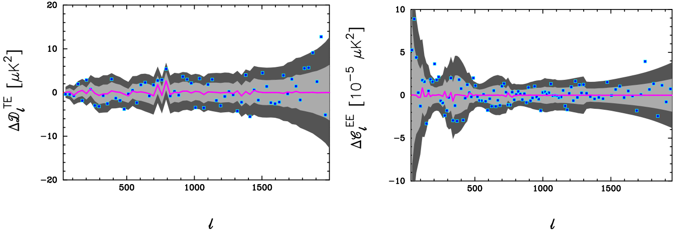
Fig. 5. Conditionals for the CamSpec TE and EE spectra, given the TT data computed from the CamSpec likelihood. As in Fig. 4, the shaded areas show \pm 1 and \pm 2\sigma ranges, computed from Eq. (16) and blue points show the residuals for the measured TE and EE spectra.
