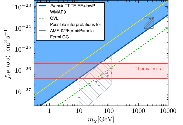
Fig. 41. Constraints on the self-annihilation cross-section at recombination, \langle\sigma v\rangle_{z_*} , times the efficiency parameter, f_{\text{eff}} (Eq. 81). The blue area shows the parameter space excluded by the Planck TT,TE,EE+lowP data at 95 % CL. The yellow line indicates the constraint using WMAP9 data. The dashed green line delineates the region ultimately accessible by a cosmic variance limited experiment with angular resolution comparable to that of Planck . The horizontal red band includes the values of the thermal-relic cross-section multiplied by the appropriate f_{\text{eff}} for different DM annihilation channels. The dark grey circles show the best-fit DM models for the PAMELA/AMS-02/ Fermi cosmic-ray excesses, as calculated in Cholis & Hooper (2013) (caption of their figure 6). The light grey stars show the best-fit DM models for the Fermi Galactic centre gamma-ray excess, as calculated by Calore et al. (2014) (their tables I, II, and III), with the light grey area indicating the astrophysical uncertainties on the best-fit cross-sections.
