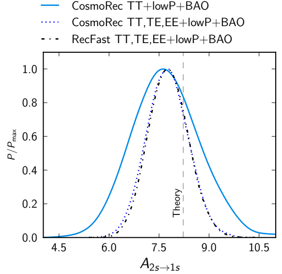
Fig. 42. Marginalized posterior for A_{2s \rightarrow 1s} , obtained using CosmoRec . We find good agreement with the theoretical value of A_{2s \rightarrow 1s} = 8.2206 \text{ s}^{-1} . For comparison, we also show the result for Planck TT,TE,EE+lowP+BAO obtained with recfast , emphasizing the consistency of different treatments.
