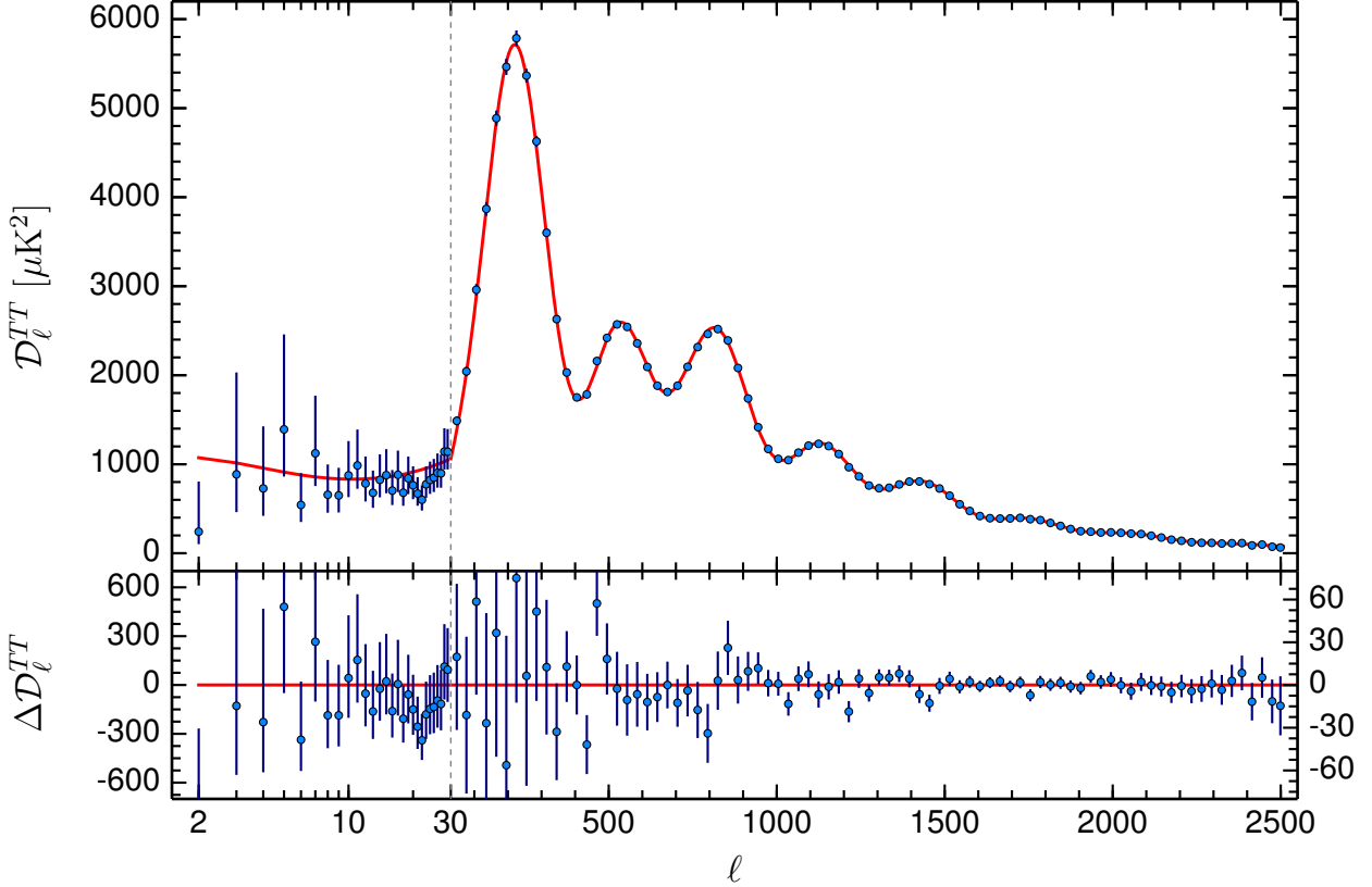
Fig. 1. The Planck 2015 temperature power spectrum. At multipoles \ell \geq 30 we show the maximum likelihood frequency averaged temperature spectrum computed from the Plik cross-half-mission likelihood with foreground and other nuisance parameters determined from the MCMC analysis of the base \Lambda CDM cosmology. In the multipole range 2 \leq \ell \leq 29 , we plot the power spectrum estimates from the Commander component-separation algorithm computed over 94% of the sky. The best-fit base \Lambda CDM theoretical spectrum fitted to the Planck TT+lowP likelihood is plotted in the upper panel. Residuals with respect to this model are shown in the lower panel. The error bars show \pm 1 \sigma uncertainties.
