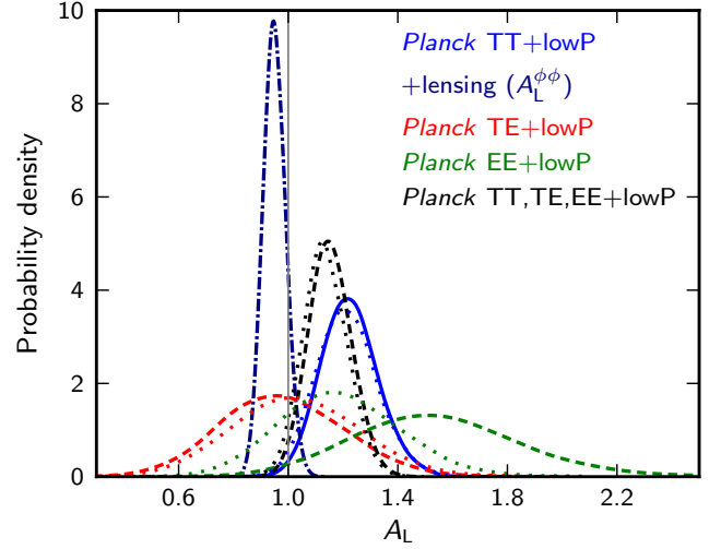
Fig. 12. Marginalized posterior distributions for measures of the lensing power amplitude. The dark-blue (dashed-dotted) line is the constraint on the parameter A_L^{\phi\phi} that scales the amplitude of the lensing power spectrum in the lensing likelihood for the Planck TT+lowP+lensing data combination. The other lines are for the A_L parameter that scales the lensing power spectrum used to lens the CMB spectra, for the data combinations Planck TT+lowP (blue, solid), Planck TE+lowP (red, dashed), Planck EE+lowP (green, dashed), and Planck TT,TE,EE+lowP (black, dashed). The dotted lines show the A_L constraints when the Plik likelihood is replaced with CamSpec, highlighting that the preference for high A_L in the Planck EE+lowP data combination is not robust to the treatment of polarization on intermediate and small scales.
