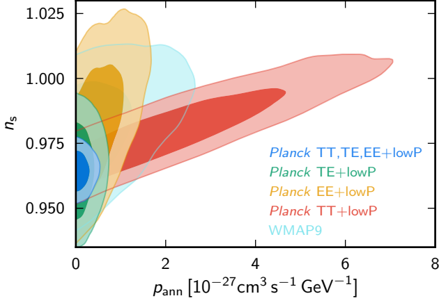
Fig. 40. 2-dimensional marginal distributions in the p_{\text{ann}}-n_s plane for Planck TT+lowP (red), EE+lowP (yellow), TE+lowP (green), and Planck TT,TE,EE+lowP (blue) data combinations. We also show the constraints obtained using WMAP9 data (light blue).
