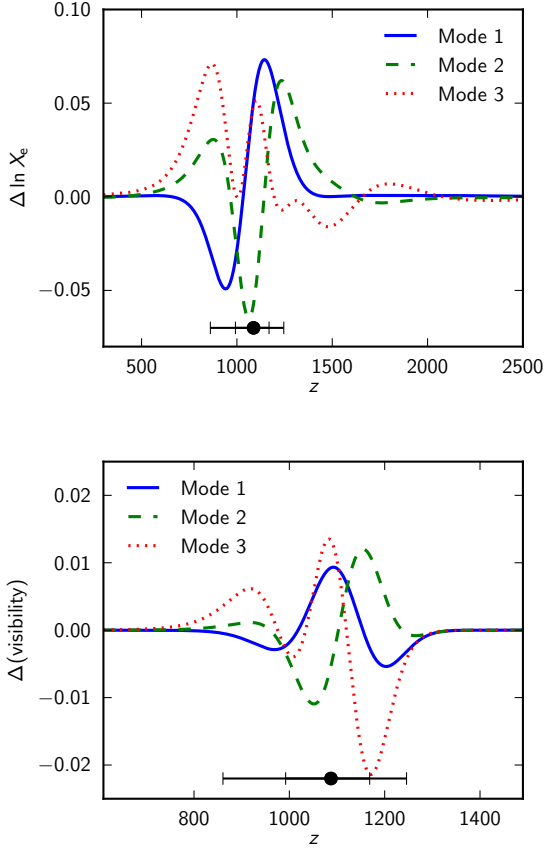
Fig. 44. Eigen-modes of the recombination history, marginalized over the standard six cosmological and Planck nuisance parameters. The upper panel shows the first three X_e -modes constructed for Planck TT,TE,EE+lowP data. The lower panel shows changes in the differential visibility corresponding to 1\sigma deviations from the standard recombination scenario for the first three X_e -modes. The maximum of the Thomson visibility function and width are indicated in both figures.
