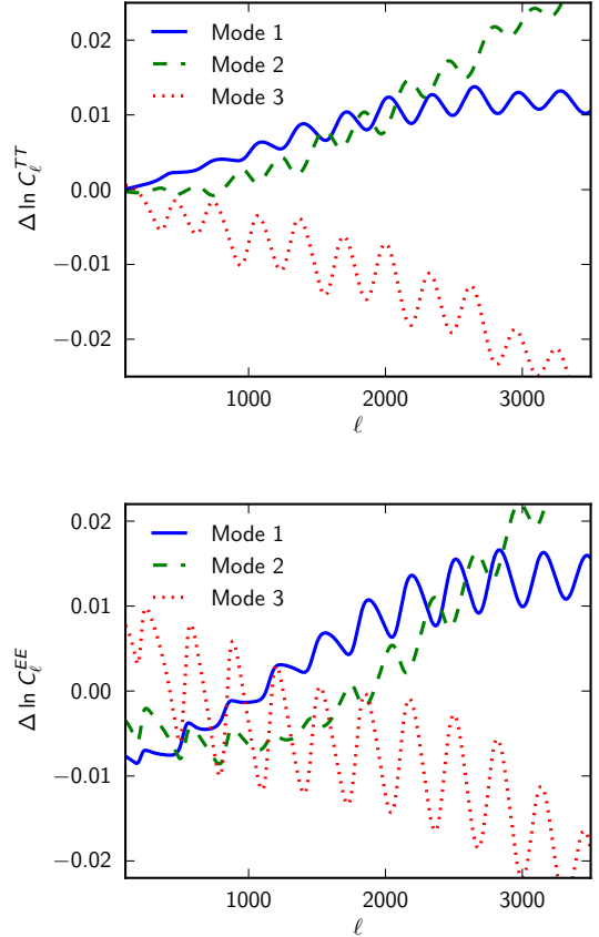
Fig. 45. Changes in the TT (upper panel) and EE (lower panel) power spectra caused by a 1\sigma deviation from the standard recombination scenario for the first three X_e -modes (see Fig. 44).
