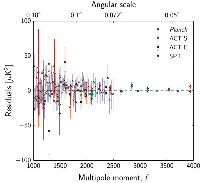
Fig. 9. Residual power with respect to the Planck TT+lowP \Lambda CDM best-fit model for the Planck (grey), ACT south (orange), ACT equatorial (red) and SPT (green) CMB bandpowers. The ACT and SPT bandpowers are scaled by the best-fit calibration factors.
