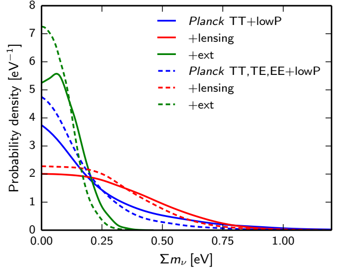
Fig. 30. Constraints on \Sigma m_\nu for various data combinations.
