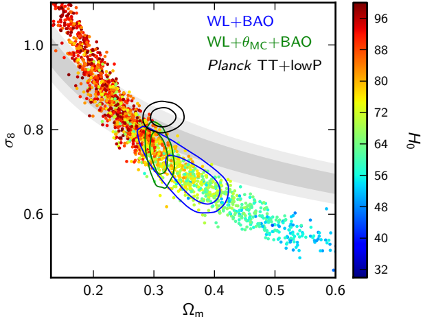
Fig. 18. Samples in the \sigma_8 – \Omega_m plane from the H13 CFHTLenS data (with angular cuts as discussed in the text), coloured by the value of the Hubble parameter, compared to the joint constraints when the lensing data are combined with BAO (blue), and BAO with the CMB acoustic scale parameter fixed to \theta_{MC} = 1.0408 (green). For comparison the Planck TT+lowP constraint contours are shown in black. The grey band shows the constraint from Planck CMB lensing.
