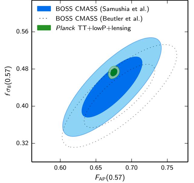
Fig. 17. 68% and 95% contours in the f\sigma_8 – F_{\text{AP}} plane (marginalizing over D_V/r_s ) for the CMASS-DR11 sample as analysed by Samushia et al. (2014) (solid, our default), and Beutler et al. (2014b) (dotted). The green contours show the constraint from Planck TT+lowP+lensing in the base \Lambda CDM model.
