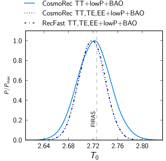
Fig. 43. Marginalized posterior for T_0 . We find excellent agreement with the COBE/FIRAS measurement. For comparison, we show the result for Planck TT,TE,EE+lowP+BAO obtained with recfast , emphasizing the consistency of different treatments.
