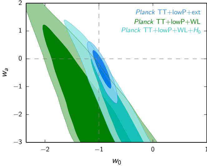
Fig. 28. Marginalized posterior distributions for (w_0, w_a) for various data combinations. We show Planck TT+lowP in combination with BAO, JLA, H_0 (“ext”), and two data combinations which add the CFHTLenS data with ultra-conservative cuts as described in the text (denoted “WL”). Dashed grey lines show the parameter values corresponding to a cosmological constant.
