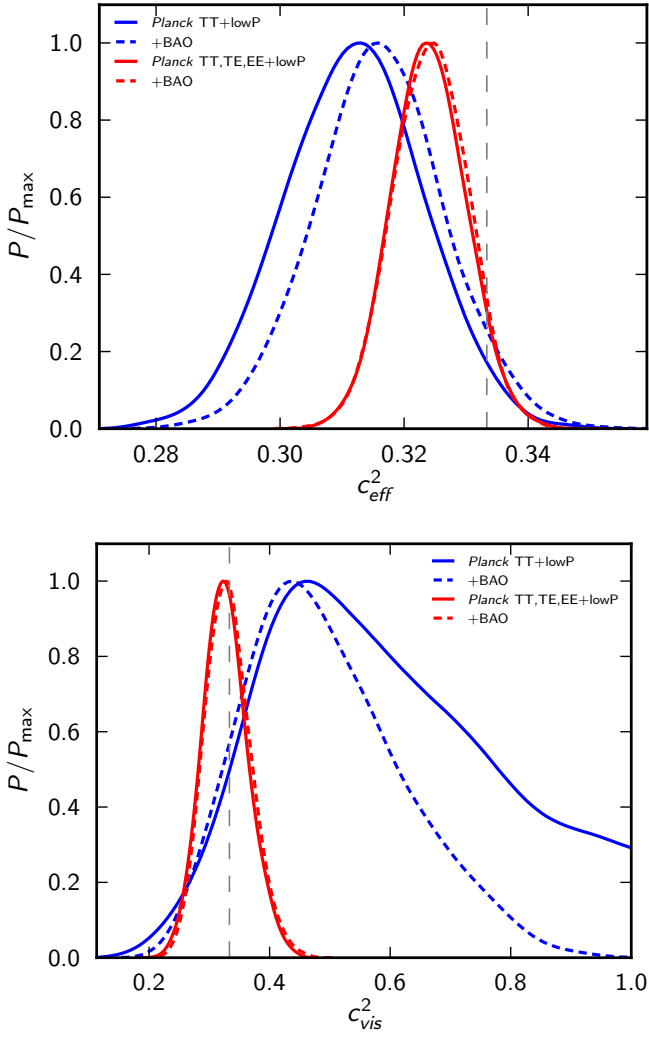
Fig. 34. 1D posterior distributions for the neutrino perturbation parameters c_{\text{eff}}^2 (top) and c_{\text{vis}}^2 (bottom). Dashed vertical lines indicate the standard values c_{\text{eff}}^2 = c_{\text{vis}}^2 = 1/3 .
