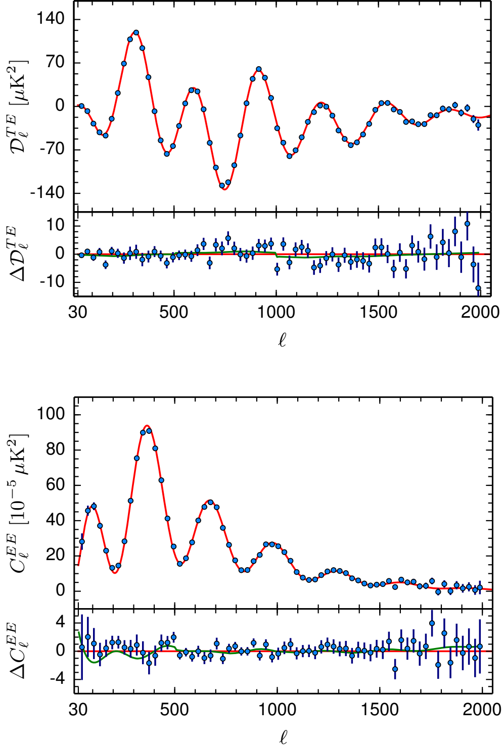
Fig. 3. Frequency-averaged TE and EE spectra (without fitting for T - P leakage). The theoretical TE and EE spectra plotted in the upper panel of each plot are computed from the Planck TT +lowP best-fit model of Fig. 1. Residuals with respect to this theoretical model are shown in the lower panel in each plot. The error bars show \pm 1\sigma errors. The green lines in the lower panels show the best-fit temperature-to-polarization leakage model of Eqs. (11a) and (11b), fitted separately to the TE and EE spectra.
