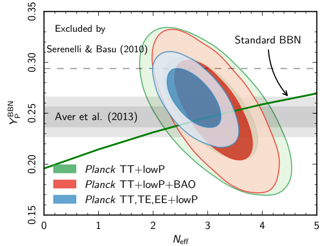
Fig. 39. As Fig. 38 but now allowing Y_p^{\text{BBN}} and N_{\text{eff}} to vary as parameter extensions to base \Lambda\text{CDM} .
