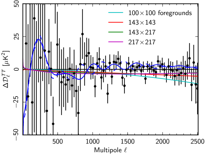
Fig. 13. Changes in the CMB TT spectrum and foreground spectra, between the best-fitting A_L model and the best-fitting base \Lambda CDM model to the Planck TT+lowP data. Blue lines show the difference between the A_L model and \Lambda CDM (solid), and the same, but with A_L set to unity (dashed) to show the changes in the spectrum arising from differences in the other cosmological parameters. Also shown are the changes in the best-fitting foreground contributions to the four frequency cross-spectra between the A_L model and the \Lambda CDM model. The data points (with \pm 1\sigma errors) are the differences between the high- \ell maximum-likelihood frequency-averaged CMB spectrum and the best-fitting \Lambda CDM model to the Planck TT+lowP data (as in Fig. 1). Note that the changes in the CMB spectrum and the foregrounds should be added when comparing to the residuals in the data points.
