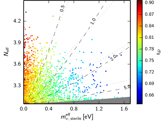
Fig. 32. Samples from Planck TT+lowP in the N_{\text{eff}}-m_{\nu,\text{sterile}}^{\text{eff}} plane, colour-coded by \sigma_8 , in models with one massive sterile neutrino family, with effective mass m_{\nu,\text{sterile}}^{\text{eff}} , and the three active neutrinos as in the base \Lambda CDM model. The physical mass of the sterile neutrino in the thermal scenario, m_{\nu,\text{sterile}}^{\text{thermal}} , is constant along the grey dashed lines, with the indicated mass in eV; the grey region shows the region excluded by our prior m_{\nu,\text{sterile}}^{\text{thermal}} < 10 eV, which excludes most of the area where the neutrinos behave nearly like dark matter. The physical mass in the Dodelson-Widrow scenario, m_{\nu,\text{sterile}}^{\text{DW}} , is constant along the dotted lines (with the value indicated on the adjacent dashed lines).
