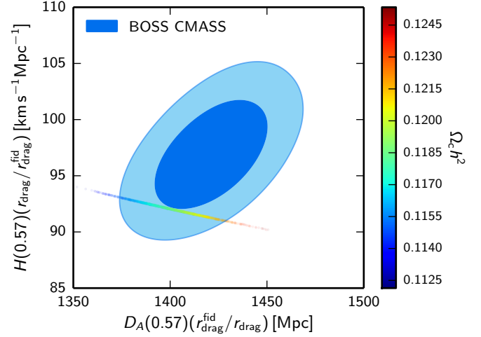
Fig. 15. 68% and 95% constraints on the angular diameter distance D_A(z = 0.57) and Hubble parameter H(z = 0.57) from the Anderson et al. (2014) analysis of the BOSS CMASS-DR11 sample. The fiducial sound horizon adopted by Anderson et al. (2014) is r_{\text{drag}}^{\text{fid}} = 149.28 Mpc. Samples from the Planck TT+lowP+lensing chains are plotted coloured by their value of \Omega_c h^2 , showing consistency of the data, but also that the BAO measurement can tighten the Planck constraints on the matter density.
