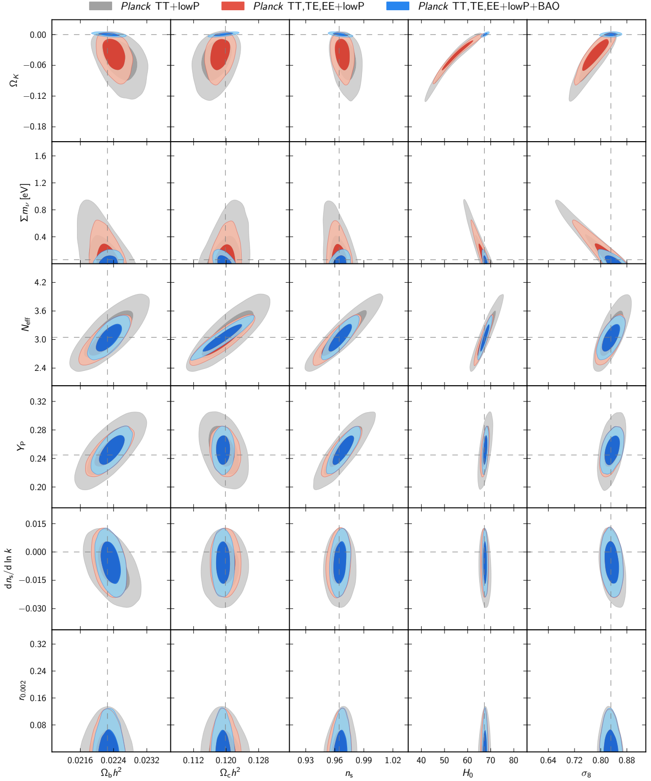
Fig. 20. 68 % and 95 % confidence regions on 1-parameter extensions of the base \Lambda CDM model for Planck TT+lowP (grey), Planck TT,TE,EE+lowP (red), and Planck TT,TE,EE+lowP+BAO (blue). Horizontal dashed lines correspond to the parameter values assumed in the base \Lambda CDM cosmology, while vertical dashed lines show the mean posterior values in the base model for Planck TT,TE,EE+lowP+BAO.
