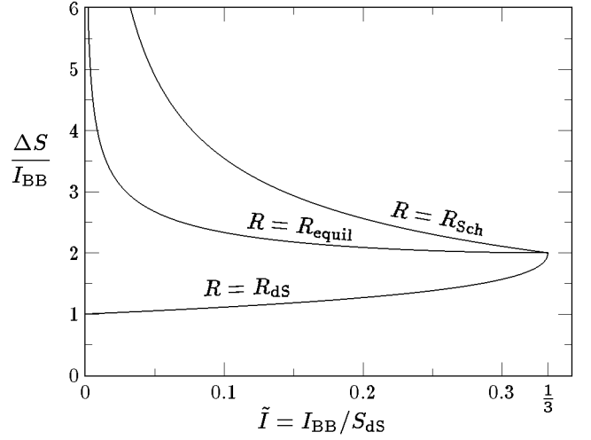
FIG. 2: Graph shows the ratio of \Delta S to I_{\text{BB}} , where the nucleation rate for Boltzmann brains is proportional to e^{-\Delta S} . All curves are based on the I-bound, as discussed in the text, but they differ by their assumptions about the size R of the Boltzmann brain.
