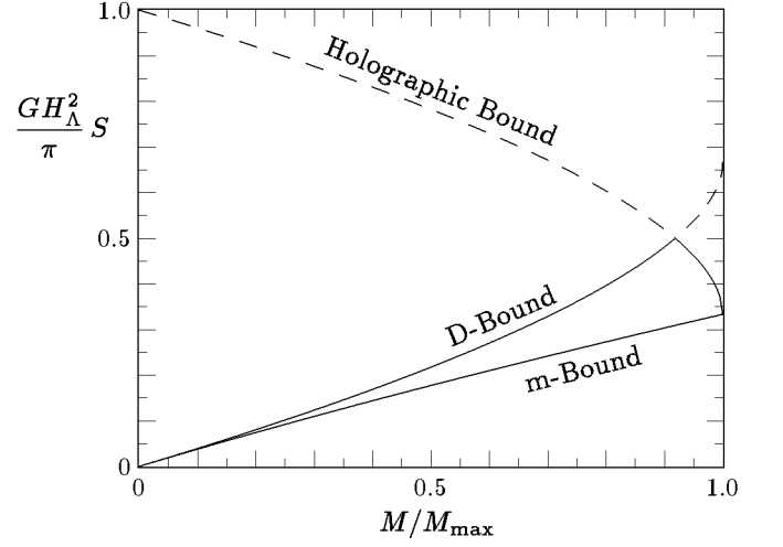
FIG. 1: Graph shows the holographic bound, the D -bound, and the m -bound for the entropy of an object that fills de Sitter space out to the horizon. The holographic and D -bounds are each shown as broken lines in the region where they are superseded by the other. Although the m -bound looks very much like a straight line, it is not.
