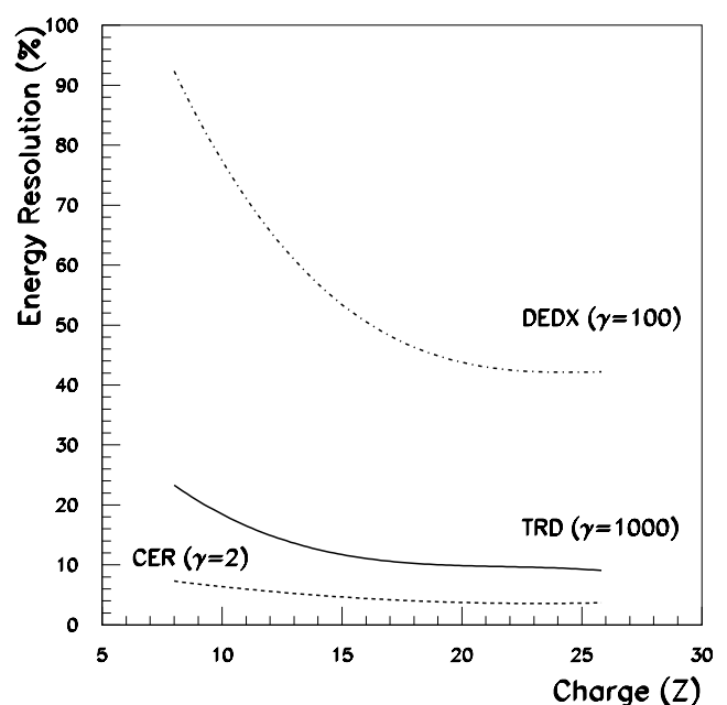
FIG. 11.—Energy resolution ( 1 \sigma ) of individual detector subsystems vs. charge Z and for typical energies: Cerenkov: \gamma = 2 (dashed line), dE/dx : \gamma = 100 (dash-dotted line), and TRD: \gamma = 1000 (solid line).
