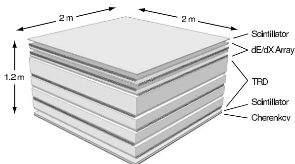
FIG. 2.—Schematic drawing of TRACER. [See the electronic edition of the Journal for a color version of this figure.]
