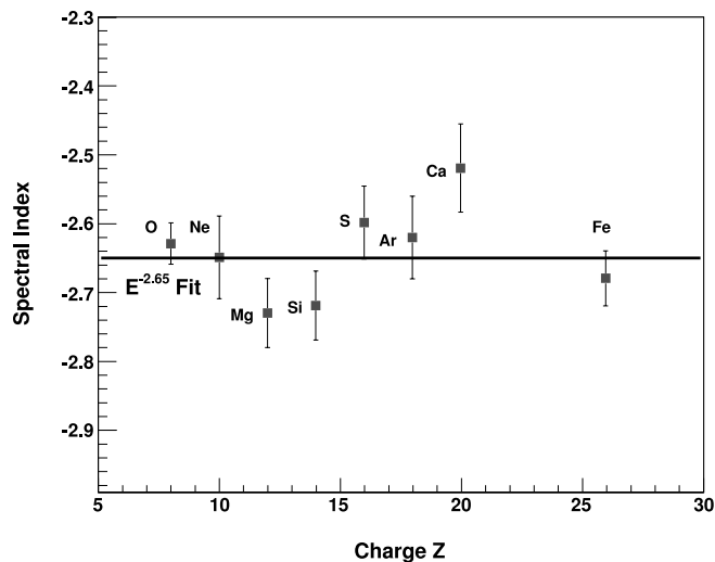
FIG. 13.—Spectral indices of a best power-law fit to the combined TRACER and CRN data above 20 GeV amu -1 . The line indicates an average spectral fit of E^{-2.65} . [See the electronic edition of the Journal for a color version of this figure.]
