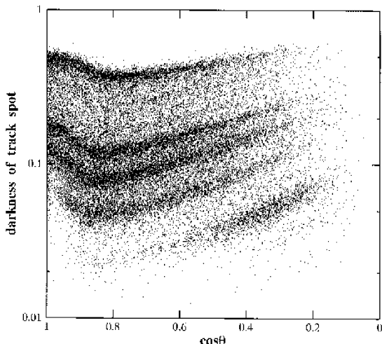
Figure 1: Scatter plot of darkness vs \cos\theta
