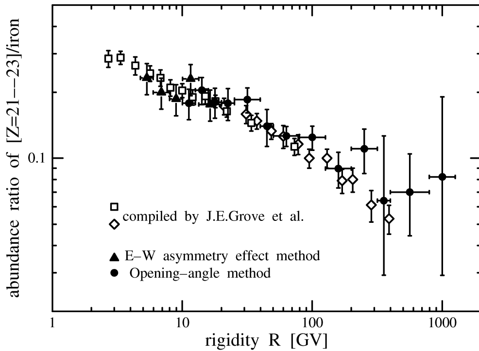
Figure 6: Abundance ratio of sub-Fe(Z=21-23) relative to Fe
