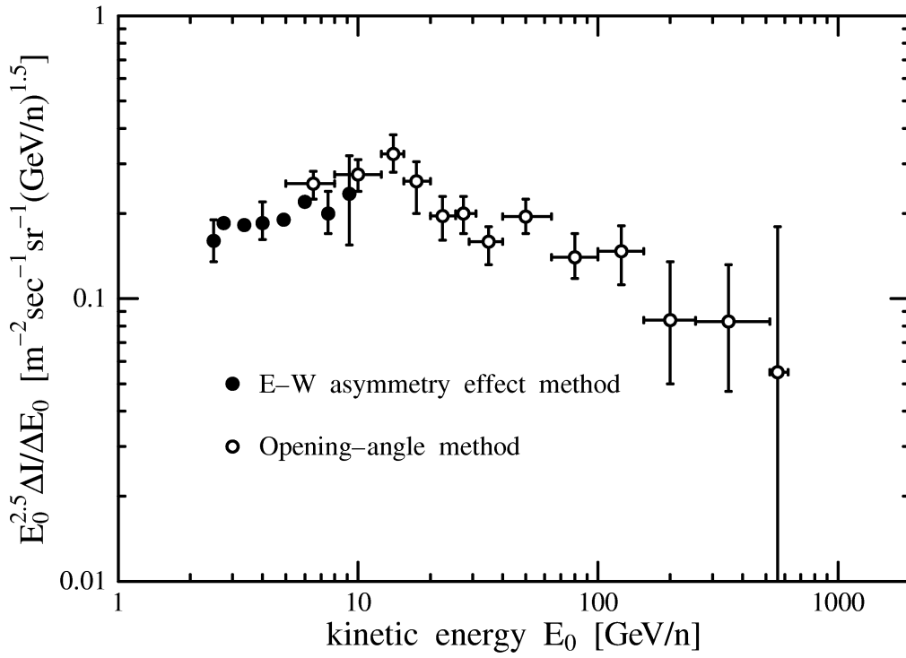
Figure 5: Absolute intensity of sub-Fe(Z=21-23)
