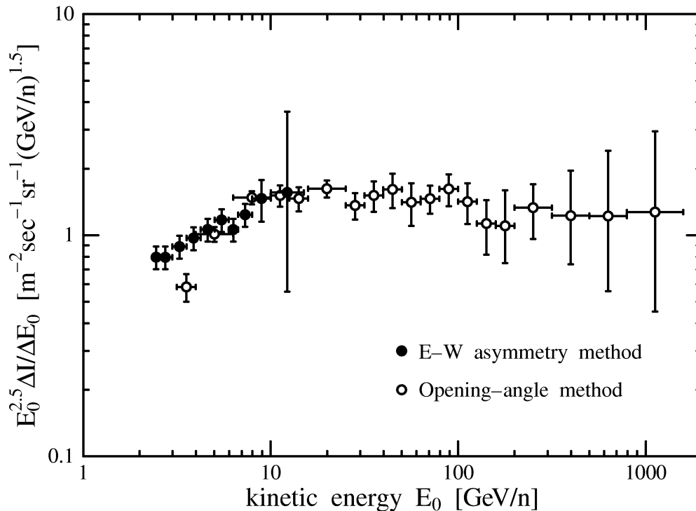
Figure 4: Absolute intensity of Fe
