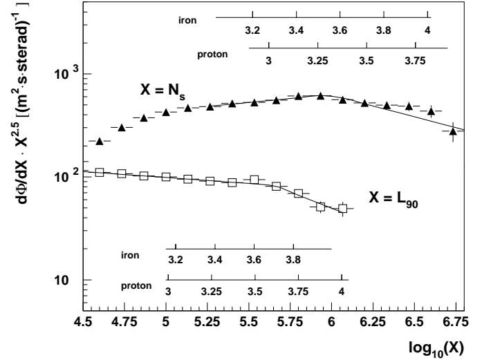
Fig. 5. The differential shower-size spectrum and “light-density at 90 m core distance ( L_{90} )” spectrum. The values used for the construction of these spectra, were employed for the energy reconstruction. The full lines indicate the best fit in the range 5.3–6.8 and 4.5–6.1 for N_s and L_{90} respectively. Two power laws which meet in a single flux value (“the knee”) were assumed. The best-fit power law indices are (-2.35/-2.92) and (-2.61/-3.13) (before/after) the knee at a position of \log_{10}(N_s)/\log_{10}(L_{90}) = 5.99/5.64 for the shower size/light density respectively. The energy scales were derived under the assumption that the primaries are all protons, resp. iron nuclei for shower size (upper scales) and light density (lower scales).
