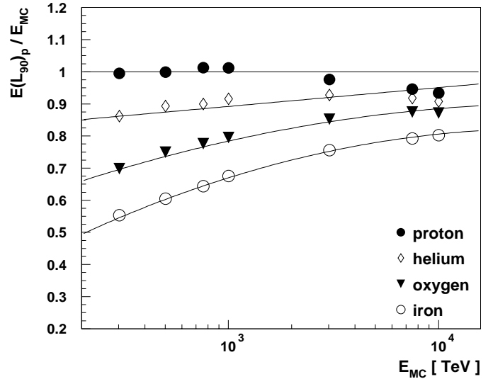
Fig. 2. The bias of the energy reconstruction as a function of primary energy for different primary masses. Shown is the ratio of the reconstructed energy with method 3, divided by the true energy (from the Monte-Carlo simulation). Very similar results are obtained from N_s and slope . The lines show fits used for convolution procedures to determine the final results (see text).
