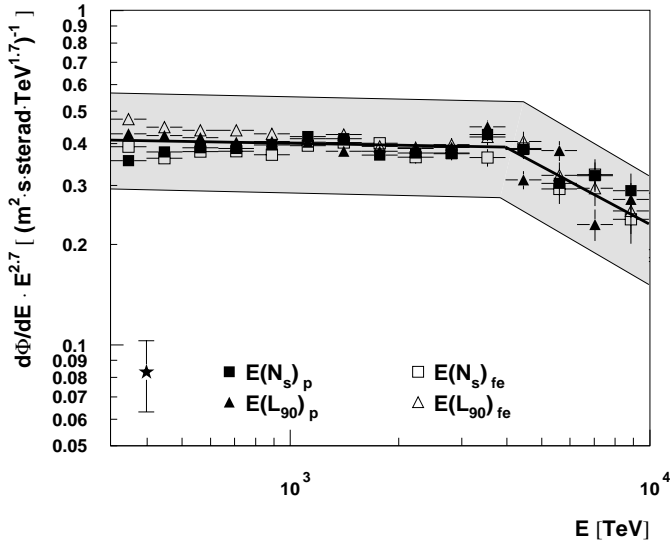
Fig. 8. The differential CR energy spectrum obtained with four energy reconstruction methods. Symbols are the same as in Fig. 6. The light shaded region represents systematical uncertainty. The “star” with vertical error bars shows the uncertainty of the HEGRA data originating from the 10% systematic uncertainty of the absolute energy scale that we estimate from the uncertainty in the determination of the absolute N_s scale. The full line is the best fit as described in the text.
