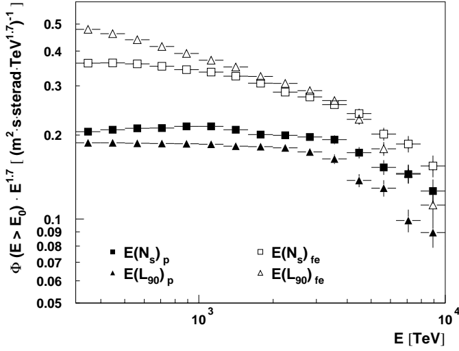
Fig. 6. The integral energy spectra obtained with the four energy reconstruction methods denoted with different symbols. Filled square: Method 1, open square: method 2, filled triangle: method 3, open triangle: method 4. The biases of the energy reconstruction have not been corrected for.
