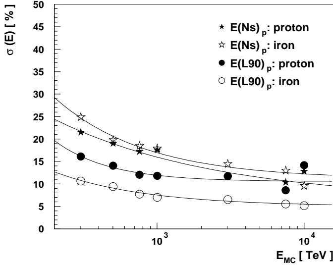
Fig. 4. The energy resolution obtained for different primary nuclei as a function of the generated MC energy. N_s in brackets denotes an energy reconstruction that combines the measured shower size at detector level and slope , L_{90} denotes the results obtained from the Cherenkov light density alone. The energy reconstruction was always performed assuming that the primaries are protons (referred to as methods 1 (stars in the figure) and 3 (dots in the figure) in the text; this fact is symbolised by the subscript “p” on the energy). The “proton” (filled symbols) “iron” (open symbols) after the colon indicate the primary for which the energy resolution was determined. The lines show fits used for convolution procedures to determine the final results (see text).
