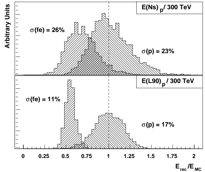
Fig. 3. Distribution of the ratio of reconstructed to MC generated energy (300 TeV) for two primaries (left distribution: iron nuclei, right distribution: protons) and the two different energy reconstruction methods discussed in the text. Each distribution is normalised to the same area.
