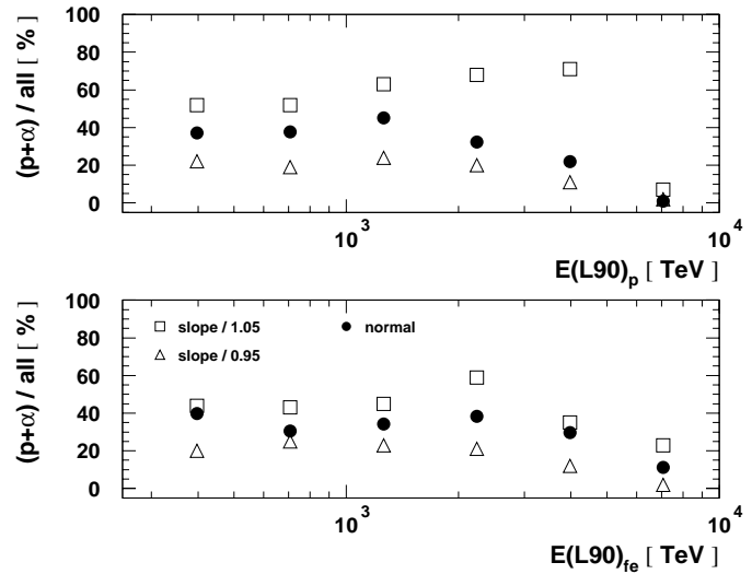
Fig. 12. The inferred chemical composition using energy-reconstruction method 3 (upper panel) and 4 (lower panel). The dots are the values as discussed before, the squares (triangles) are the results obtained when the slope is increased (decreased) by 5 % (the systematic error on this variable). The general “trend” (composition gets heavier/lighter) may change within this systematics.
