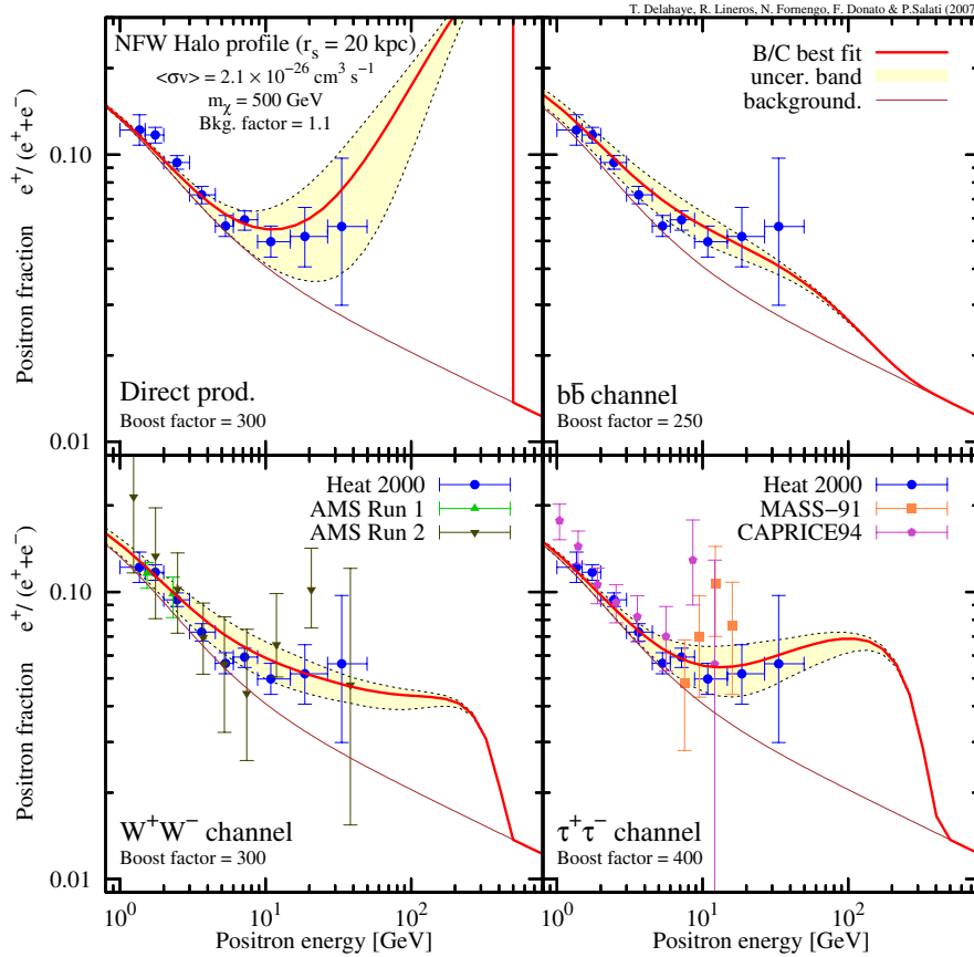
FIG. 12 (color online). Same plot as in Fig. 11 but with a mass of the DM particle of 500 GeV.
