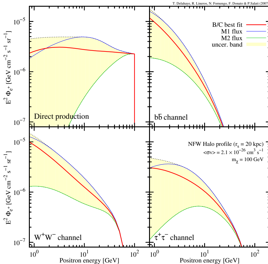
FIG. 7 (color online). Positron flux E^2\Phi_{e^+} versus the positron energy E , for a DM particle with a mass of 100 GeV and for a NFW profile—see Table I. The four panels refer to different annihilation final states : direct e^+e^- production (top left), b\bar{b} (top right), W^+W^- (bottom left), and \tau^+\tau^- (bottom right). In each panel, the thick solid [red] curve refers to the best-fit choice (MED) of the astrophysical parameters. The upper [blue] and lower [green] thin solid lines correspond, respectively, to the astrophysical configurations which provide here the maximal (M1) and minimal (M2) flux—though only for energies above a few GeV in the case of (M1). The colored [yellow] area features the total uncertainty band arising from positron propagation.
