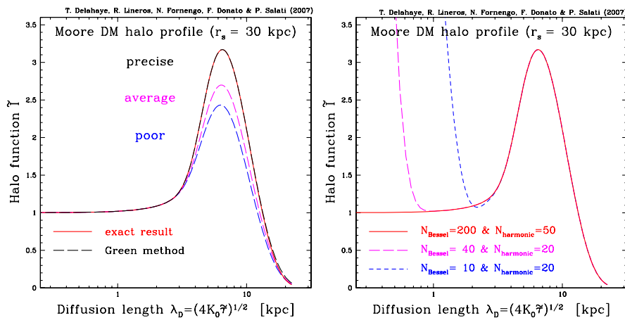
FIG. 3 (color online). The halo integral \tilde{I} is plotted as a function of the diffusion length \lambda_D in the case of a Moore profile with L = 10 kpc. In the left panel, the results obtained with the Green function method are featured by the long-dashed curves and may be compared to the exact solution and its solid red line. In the right panel, the numbers N_{\text{Bessel}} and N_{\text{harmonic}} of the eigenfunctions considered in the Bessel expansion (28) have been varied. The various curves reproduce astonishingly well the bump but diverge at small \lambda_D when too few Bessel and Fourier terms are considered.
