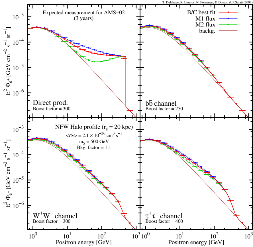
FIG. 15 (color online). Predictions for AMS-02 for a 3-year mission. The positron flux E^2\Phi_{e^+} and its statistical uncertainty are featured as a function of the positron energy E for a 500 GeV DM species and a NFW profile. Notations are the same as in Fig. 13. The thick solid curves refer, respectively, to the total positron flux calculated with the M1 (upper [blue]), MED (median [red]), and M2 (lower [green]) sets of propagation parameters.
