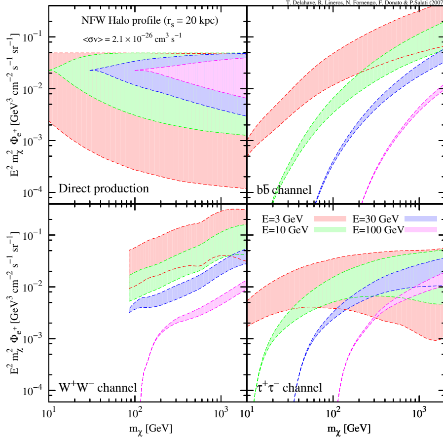
FIG. 10 (color online). For fixed values of the detected energy E , the uncertainty bands on the positron flux E^2 m_\chi^2 \Phi_{e^+} are shown as a function of the mass m_\chi of the DM particle. The energies considered in the figure are E = 3, 10, 30, and 100 GeV. Each band refers to one of those values and starts at m_\chi = E .
