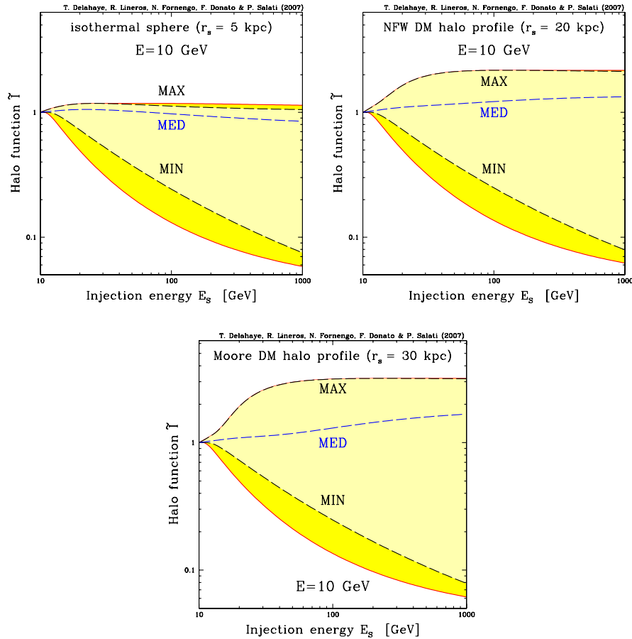
FIG. 5 (color online). In each panel, the halo integral \tilde{I} is plotted as a function of the positron injection energy E_S whereas the energy E at the Earth is fixed at 10 GeV. The galactic DM halo profiles of Table I are featured. The curves labeled as MED correspond to the choice of cosmic ray propagation parameters which best-fit the B/C ratio [12]. The MAX and MIN configurations correspond to the cases which were identified to produce the maximal and minimal DM antiproton fluxes [25], while the entire colored band corresponds to the complete set of propagation models compatible with the B/C analysis [12].
