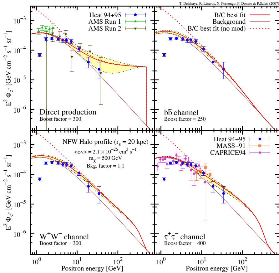
FIG. 13 (color online). Positron flux E^2\Phi_{e^+} (not fraction) versus the positron energy E , for a 500 GeV DM particle. Notations are the same as in Fig. 11. Experimental data from HEAT [2], AMS [4,5], CAPRICE [6], and MASS [7] are plotted.
