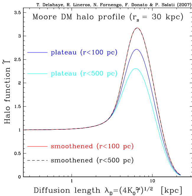
FIG. 4 (color online). Same plot as before where the central DM profile within a radius r_0 is either a plateau at constant density \rho_0 or the smooth distribution \rho^* of Eq. (29). In the former case, the bump which \tilde{I} exhibits is significantly underestimated even for values of r_0 as small as 100 pc—solid dark blue—and drops as larger values are considered—solid light blue. On the contrary, if the DM cusp is replaced by the smooth profile \rho^* , the halo integral no longer depends on the renormalization radius r_0 and the solid red and long-dashed black curves are superimposed on each other.
