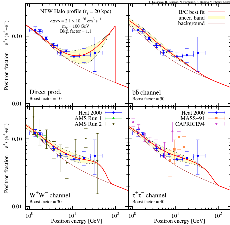
FIG. 11 (color online). Positron fraction e^+/(e^- + e^+) versus the positron detection energy E . Notations are as in Fig. 7. In each panel, the thin [brown] solid line stands for the background [1,8] whereas the thick solid [red] curve refers to the total positron flux where the signal is calculated with the best-fit choice (MED) of the astrophysical parameters. Experimental data from HEAT [2], AMS [4,5], CAPRICE [6], and MASS [7] are also plotted.
