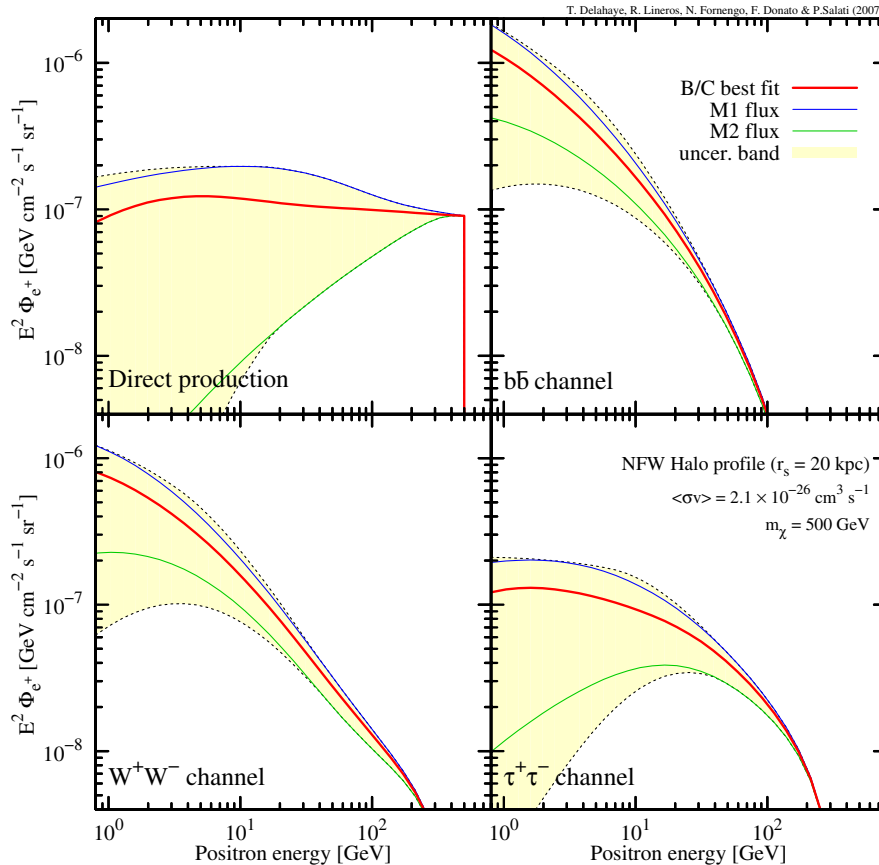
FIG. 8 (color online). Same plot as in Fig. 7 but with a DM particle mass of 500 GeV.
