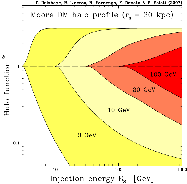
FIG. 6 (color online). Same plot as before where the Moore DM profile has been selected. Four values of the positron detection energy E have been assumed. The flag-like structure of this figure results from the widening of the uncertainty band as the detection energy E is decreased.
