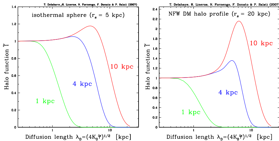
FIG. 2 (color online). The halo convolution \tilde{I} is plotted as a function of the diffusion length \lambda_D for various values of the slab half-thickness L . The left panel features the case of an isothermal DM distribution whereas a NFW profile has been assumed in the right panel—see Table I. When L is large enough for the positron horizon to reach the galactic center and its denser DM distribution, a maximum appears in the curves for \lambda_D \sim r_\odot .
