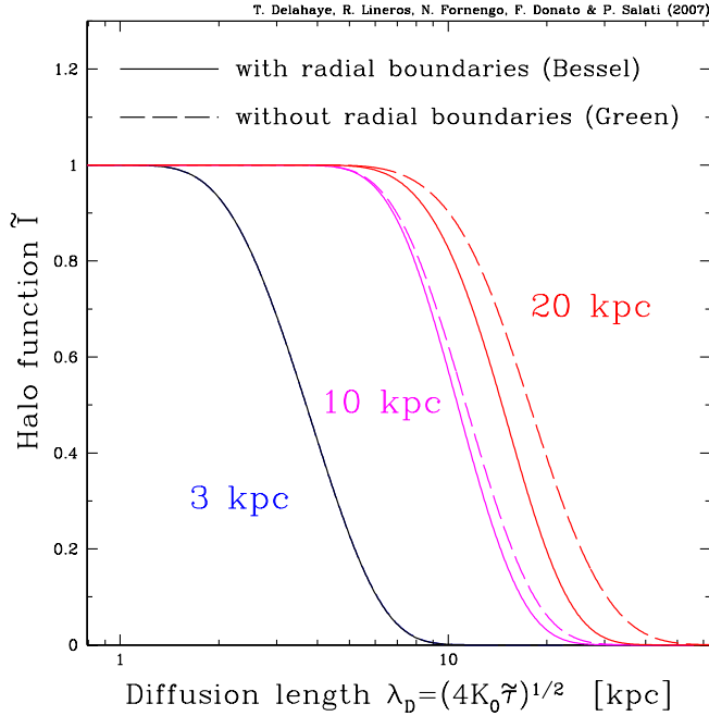
FIG. 1 (color online). Influence of the radial boundary condition for a slab half-thickness L of 3, 10, and 20 kpc ( R_{\text{gal}} = 20 kpc). The thicker the slab, the larger the error when neglecting the radial boundary. On the contrary, for small values of L , positrons produced near the radial outskirts of the diffusive halo escape into the intergalactic medium and do not contribute to the signal at the Earth. Implementing correctly the radial boundary condition is not relevant in that regime.
