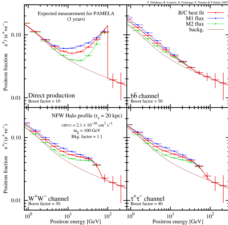
FIG. 14 (color online). Predictions for PAMELA for a 3-year mission. The positron fraction e^+/(e^- + e^+) and its statistical uncertainty are plotted against the positron energy E for a 100 GeV DM particle and a NFW profile. Notations are the same as in Fig. 11. The thick solid curves refer, respectively, to the total positron flux calculated with the M1 (upper [blue]), MED (median [red]), and M2 (lower [green]) sets of propagation parameters.
