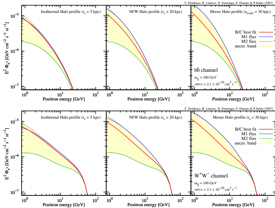
FIG. 9 (color online). Positron flux E^2 \Phi_{e^+} versus the positron energy E , for a DM particle mass of 100 GeV and for different halo density profiles: cored isothermal sphere [21] (left panels), NFW [22] (central panels), and Moore [23] (right panels)—see Table I. The upper and lower rows correspond, respectively, to a b\bar{b} and W^+W^- annihilation channel. In each panel, the thick solid [red] curve refers to the best-fit choice (MED) of the astrophysical parameters. The upper [blue] and lower [green] thin solid lines stand for the astrophysical configurations M1 and M2 of Table III. The colored [yellow] area indicates the total uncertainty band arising from positron propagation.
