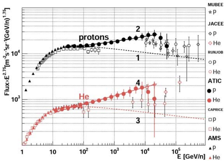
Figure 5. Proton and helium spectra measured in ATIC-2 compared to earlier measurements [8]. Lines correspond to predictions from Leaky Box model (1 and 3) and diffusion model with reacceleration (2 and 4).
