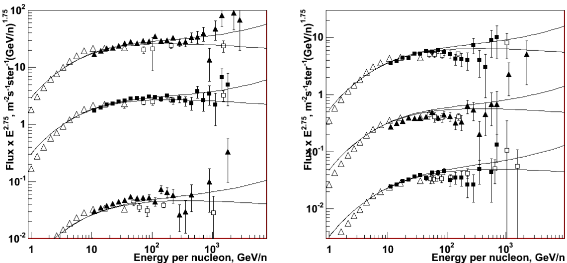
Figure 6. Energy spectra of abundant nuclei from ATIC-2 ( \blacktriangle and \blacksquare ). Left hand side: Data from top to bottom are for C, O/10, and Ne/100. Right hand side: Data from top to bottom are for Mg, Si/10, and Fe/100. Also shown are results from HEAO-3-C2 ( \triangle ) and CRN ( \square ).
