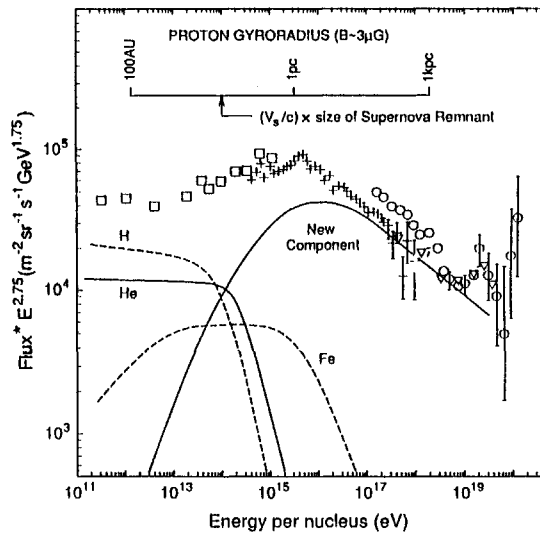
Figure 1. Sketch of the spectra expected for individual cosmic ray species in the standard supernova shock acceleration model [2]. The H, He, and Fe spectra are predicted to steepen near 10^{14} eV. The points show a sample of satellite and ground-based measurements of the all-particle spectrum. A schematic “new component” is needed to account for the observed flux above the expected galactic supernova cutoff.
