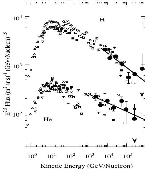
Figure 2. JACEE 1-12 differential spectra for H and He together with earlier results [3].
