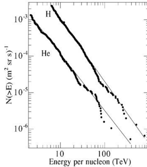
Figure 3. JACEE 1-12 integral spectra for hydrogen and helium.
