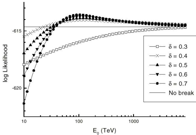
Figure 7. Log likelihood of a steepening in the JACEE proton spectrum by \delta in the power law spectral index at a break energy E_0
