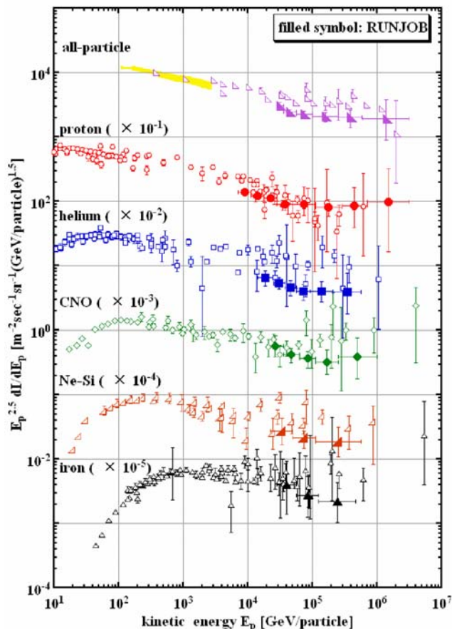
Figure 4. Final hydrogen - iron spectra obtained by RUNJOB (solid points) compared to other measurements and the all-particle spectrum [6]. In particular, note that the absolute proton intensities reported by RUNJOB (●) and JACEE (○) are in reasonable agreement while the helium intensities (■ and □ respectively) differ by approximately a factor of 2.
