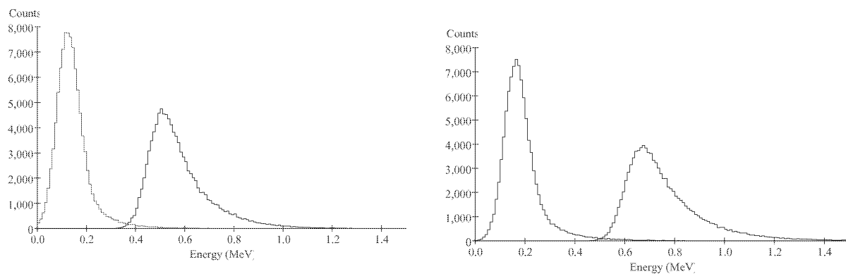
Figure 6. The average of the energy deposition in the first and second pixel encountered at 10 TeV/nucleon including 58 keV of electronic noise. Distribution for both protons and helium nuclei are shown. (The left plot is for normal incidence and the right plot is for 40° incidence.)
