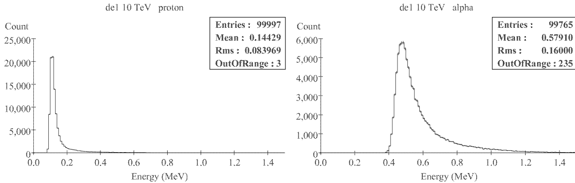
Figure 3. Energy deposition in the first silicon pixel encountered at a primary particle kinetic energy of 10 TeV/nucleon. The left graph is for protons, and the right graph is for helium nuclei.
