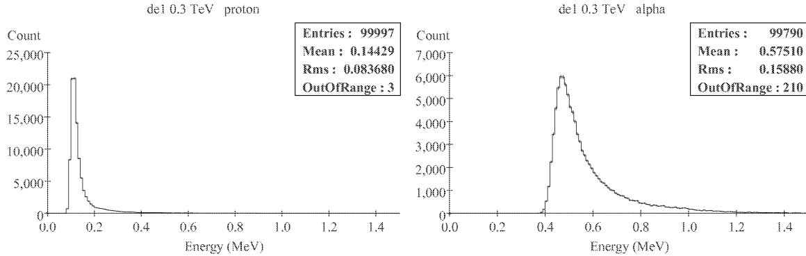
Figure 2. Energy deposition in the first silicon pixel encountered at a primary particle kinetic energy of 0.3 TeV/nucleon. The left graph is for protons, and the right graph is for helium nuclei.
