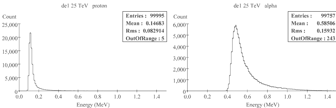
Figure 4. Energy deposition in the first silicon pixel encountered at a primary particle kinetic energy of 25 TeV/nucleon. The left graph is for protons, and the right graph is for helium nuclei.
