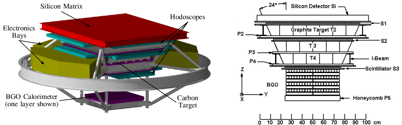
Fig. 1. 3D mechanical drawing and 2D simulation schematic of the ATIC configuration.
